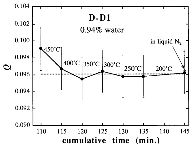
Appendix Fig. 1. Examination of whether or not there is a subreaction of Reaction 1 that has a T_{\text{re}}^* below 450 °C. Sample D-D1 contains 0.94% total water. Error bar is 2.6% (relative) of the value. The first point shows that measurement after equilibrium is established at 500 °C (110 min). The sample was heated sequentially for 5 min each at 450, 400, 350, 300, and 250 °C, and for 10 min at 200 °C. The temperature for each time interval is marked. The point that follows the temperature is the speciation measured after heating at the temperature. Solid circles = measurement of quenched glass at room temperature, and open circle = in situ measurement in liquid N 2 .
