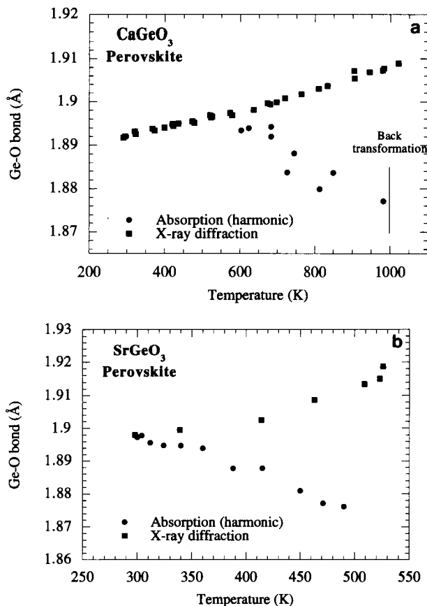
FIGURE 8. Temperature variation of the Ge-O bond length in (a) \text{CaGeO}_3 , and (b) \text{SrGeO}_3 perovskites using a classical harmonic model. The discrepancy between the absorption and diffraction results is due to the increase of the Ge-O bond anharmonicity.
