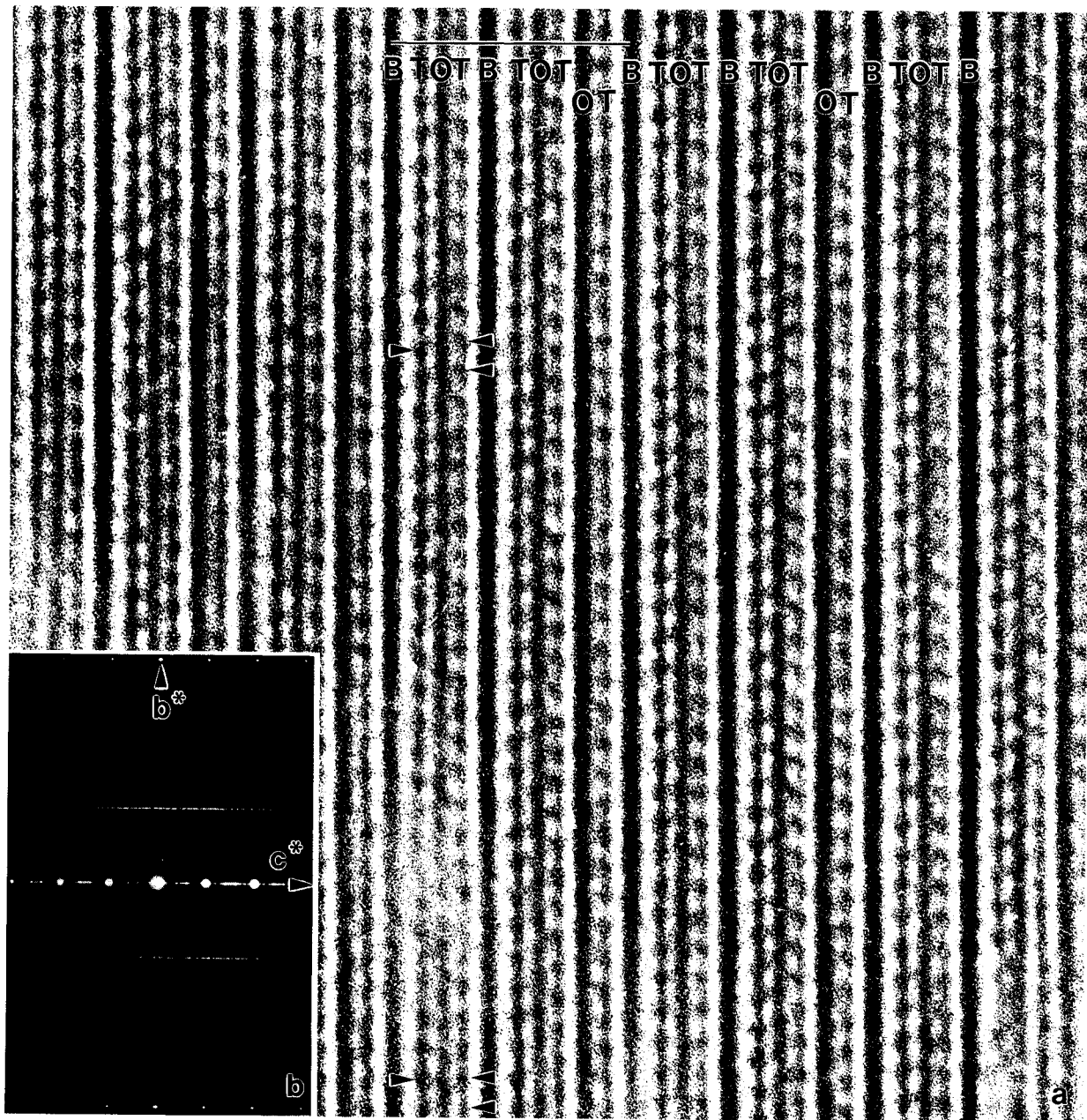
FIGURE 6. (a) HRTEM structural image down [100] illustrating an area composed primarily of regularly interstratified S_2C_2 . A dozyite defect is present to the left of the single arrows. Electron-beam damage is focused where a 2:1 layer with +b/3 shift passes into a layer with zero shift (see arrows). (b) SAED pattern for a illustrating a 3.5 nm periodicity in 00/ and intensities similar to those shown in Figure 5b. Note the continuous streaking of 0kl , k \neq 3n , indicating no true periodicity for basal O atoms along c^* (semirandom stacking).
