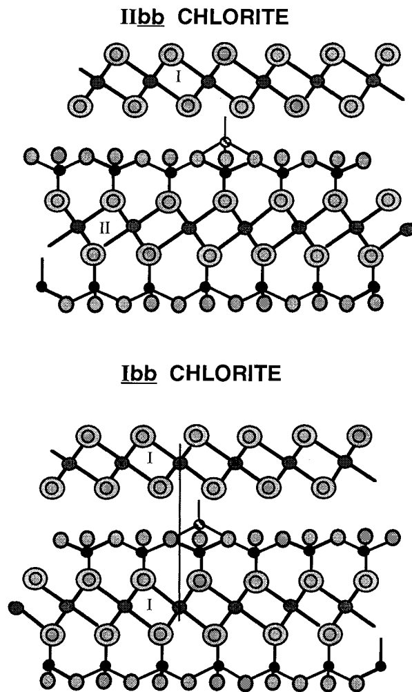
FIGURE 14. Diagram down [010] showing that if conversion of the common IIbb and less common Ibb chlorite polytypes to serpentine occurs by tetrahedral inversion, tetrahedral cations and associated O atoms must shift parallel to a to achieve an appropriate coordination environment and hydrogen bonding. In the case of inversion in IIbb chlorite, the argument regarding type-a vs. type-b interactions given for Figure 13 may result in production of lizardite-1 T . For Ibb chlorite, lizardite-1 T can be produced by translation of Si and basal O without restructuring the octahedral portion of the new 1:1 layer.
