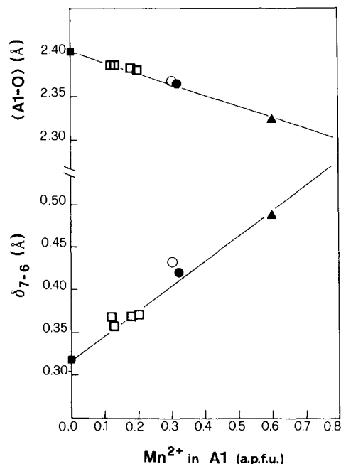
FIGURE 1. Parameters of the A1 polyhedron as a function of the Mn 2+ content of A1. Average of the six smallest A1-O distances is designated <A1-O>; the equation of the regression line is: y = 2.404 - 0.135x ( r = -0.993 ). Difference between the seventh (A1-O6) and the sixth largest (A1-O5) distances is designated \delta_{7-6} ; the equation of the regression line is y = 0.321 + 0.280x ( r = 0.990 ). Solid and open squares represent piemontite from Saint Marcel (Dollase 1969) and REE-bearing piemontite crystals, respectively [BR1A, BR2P, BR2H (Bonazzi et al. 1992), BR1P (authors' unpublished data)]; solid circles represents VA1-a and solid triangles AND-517; open circles represent the sample from Nezilovo (Bermanec et al. 1994), for which a content of Mn_{A1}^{2+} = 0.30 apfu was assumed (see text).
