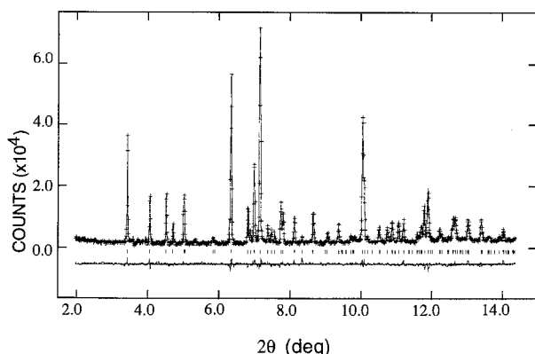
FIGURE 1. Calculated (continuous line) and observed (crosses) synchrotron X-ray diffraction profiles for (Ni 0.5 Mg 0.5 ) 2 SiO 4 olivine at 4 GPa and 800 °C. A difference curve ( I_{\text{obs}} - I_{\text{calc}} ) is plotted at the bottom on the same scale. Allowed reflection positions are indicated by vertical lines.
