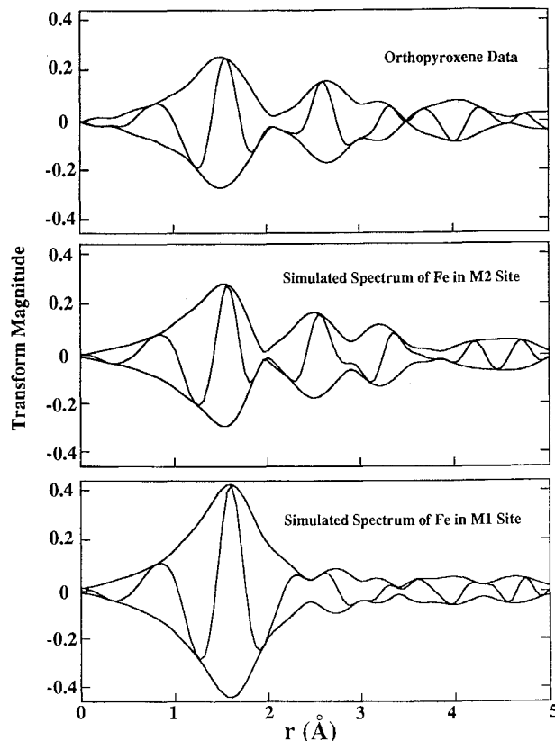
FIGURE 3. Fourier transforms of the XAFS data and synthetic XAFS spectra for Fe in the M1 and M2 sites. The outer envelope is the magnitude of the FT [ \pm(\text{Re}^2 + \text{Im}^2)^{1/2} ], and the inner curve represents the real part of the transform. Note that the zero crossings of the inner curve closely match those of the data and M2 synthetic spectra out to 2.2 Å. The bond distances plotted here were uncorrected for phase shift and so are ~0.5 Å shorter than the actual bond lengths.
