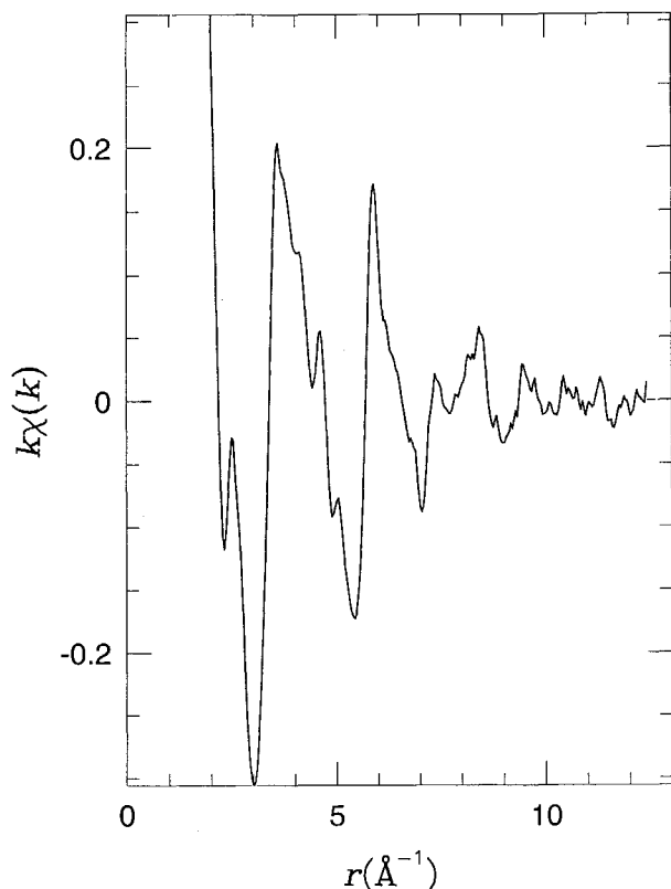
FIGURE 2. XAFS data of the k space at the Fe K edge in (Mg,Fe)SiO 3 enstatite.
