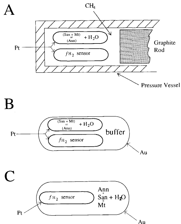
FIGURE 2. Capsule configurations used in this study. (A) CH 4 pressure medium and a graphite filler rod making up the buffer, plus an f_{\text{H}_2} sensor and the experimental charge in platinum capsules containing either annite (Ann) + H 2 O or sanidine (San) + magnetite (Mt) + H 2 O. (B) The traditional hydrothermal method of redox control using a double-tube technique with the addition of an f_{\text{H}_2} sensor. (C) The setup primarily used for the low-temperature experiments. Consists of the complete Ann + San + Mt + H 2 O assemblage and an f_{\text{H}_2} sensor. The f_{\text{H}_2} sensor was constructed of very thin walled (0.1 mm) platinum.
