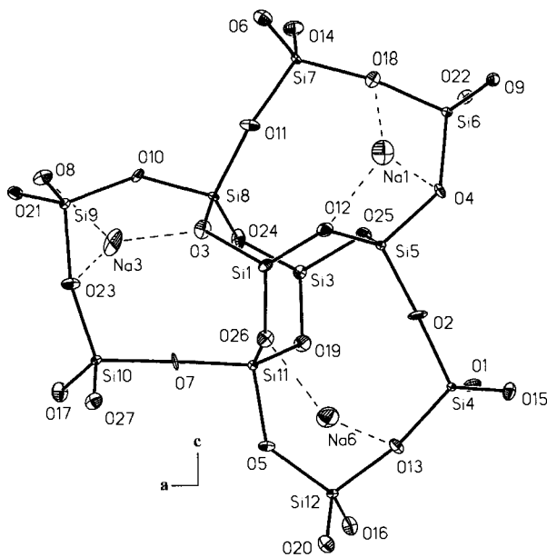
FIGURE 1. Nine-membered rings of independent \text{SiO}_4 tetrahedra in the structure of \text{Na}_6\text{Si}_3[\text{Si}_9\text{O}_{27}] gathered by O3, O12, and O26 of the \text{Si1O}_6 octahedron and O19, O24, and O25 of the \text{Si3O}_6 octahedron. Note that the vibrational ellipsoids were determined at room temperature and pressure.
