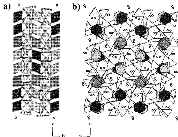
FIGURE 2. Polyhedral representations of the structure of \text{Na}_6\text{Si}_3[\text{Si}_9\text{O}_{27}] viewed along [100] (a) and [010] (b). Shading of octahedra is light for \text{Si1O}_6 , moderate for \text{Si2O}_6 , and heavy for \text{Si3O}_6 . Open circles are Na positions. Note that the layers of collapsed nine-membered rings of \text{SiO}_4 tetrahedra are in ABA-B... packing along [010]. Also, octahedra, interspersed with unoccupied trigonal prisms, form columns along [010], with alternating \text{Si1O}_6 and \text{Si3O}_6 in one column and \text{Si2O}_6 alone in another.
