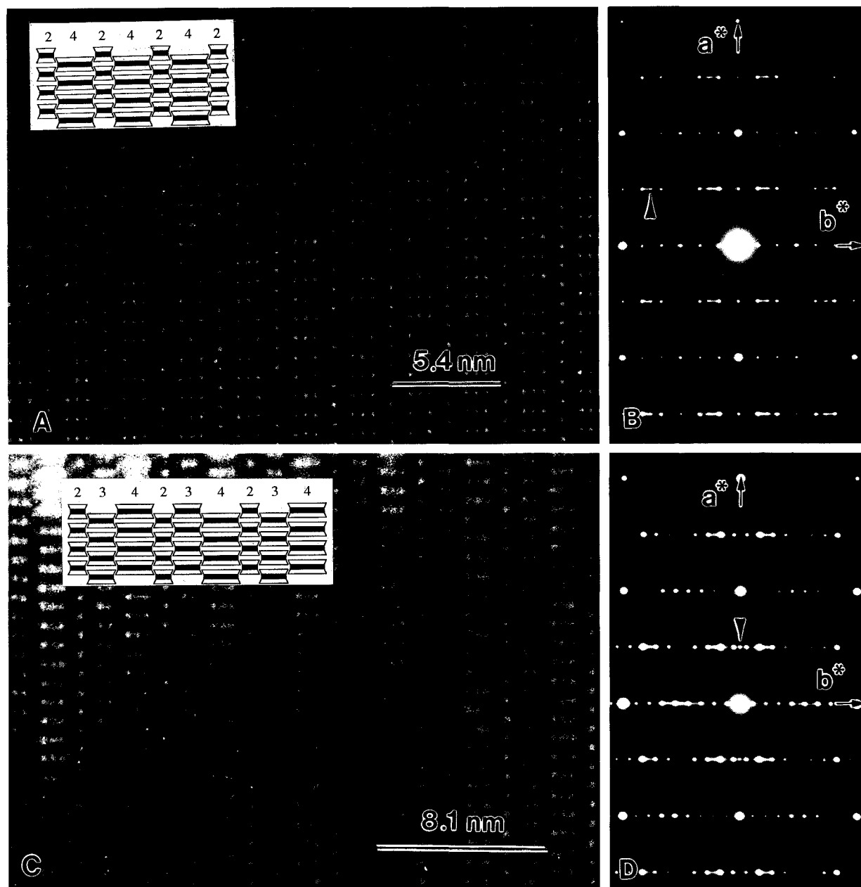
FIGURE 2. HRTEM images and SAED patterns of the [001] zone of the polysome (42) (A and B) and the polysome (234) (C and D). The insets in the images are 1-beam representations of the polysomes with the numbers of subchains in each Si tetrahedral chain indicated on top. The arrows in B and D point to diffraction spots belonging to anthophyllite.
