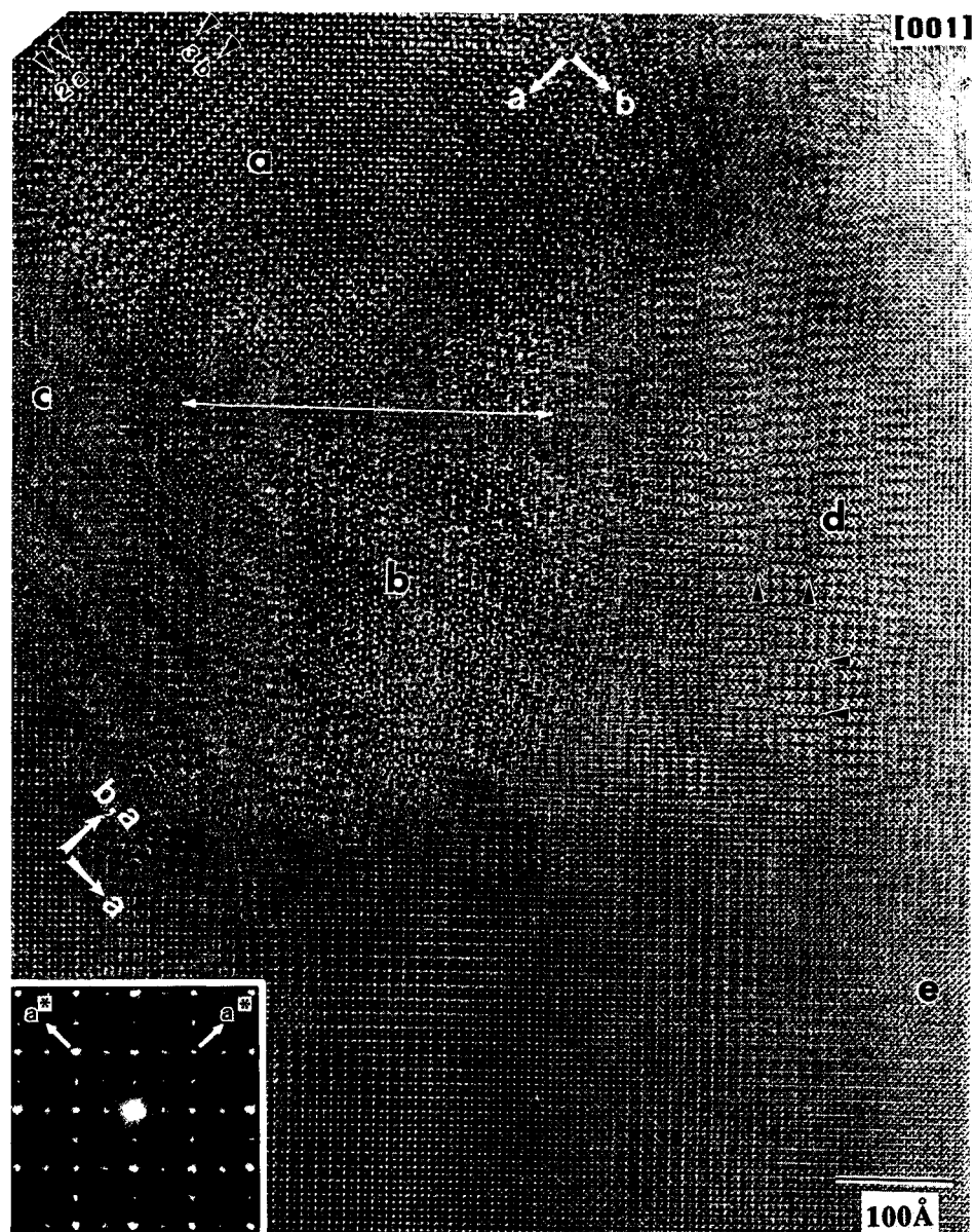
FIGURE 5. The [001] image of aluminite sodalite after transformation. The twin boundary is indicated by the double-headed arrow. Region a contains a 2a \times 3b supercell that did not change during the transformations. Regions b and c contain modulated fringes, region d contains two-dimensional periodic APBs (pairs of arrows), and region e is a product of the transformation and has tetragonal symmetry, as indicated by the optical diffractogram (inset).
