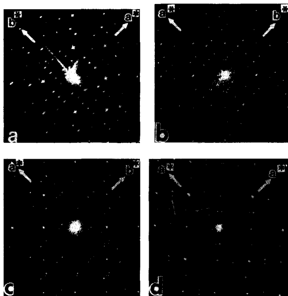
FIGURE 6. Optical diffractograms of the regions shown in the [001] image of aluminite sodalite (Fig. 5). Diffractograms a–d correspond to the regions labeled a–d in Figure 5. A 2a \times 3b supercell is shown in a , b and c indicate modulations along b^* , and the arrows in d point to r_s reflections that cause the two-dimensional periodic APBs.
