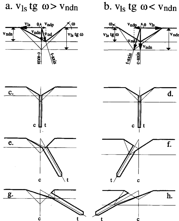
FIGURE 22. Diagram showing different etch-pit profiles in \{0001\} , depending on the values of v_{ls} , v_{ndn} , and \omega and on the angle of incidence, \theta , of the fission track; (a) \tan \omega > v_{ndn}/v_{ls} , (b) \tan \omega < v_{ndn}/v_{ls} , (c) \theta = 90^\circ , (d) \theta = 90^\circ , (e) \tan \theta > v_{ndn} \tan \omega / (v_{ls} \tan \omega - v_{ndn}) , (f) \tan \theta > v_{ndn} \tan \omega / (v_{ndn} - v_{ls} \tan \omega) , (g) \tan \theta < v_{ndn} \tan \omega / (v_{ls} \tan \omega - v_{ndn}) , (h) \tan \theta < v_{ndn} \tan \omega / (v_{ndn} - v_{ls} \tan \omega) .
