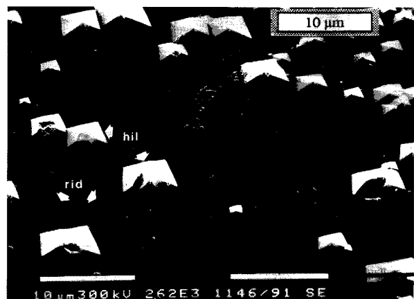
FIGURE 13. The texture on \{10\bar{1}0\} (T type) is made up of two components. The fundamental texture consists of parallel ridges (rid) separated by grooves and is clearly distinguishable from the pointed hillocks (hil) that make up the superimposed texture. Etching conditions: 1800 s in 2.5% \text{HNO}_3 (set B).
