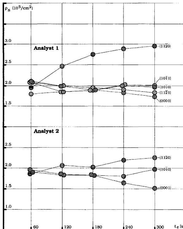
FIGURE 23. Evolution of the spontaneous track density ( \rho_s ) in the {0001}, {1010}, {1120}, {1011}, and {1121} sections of Durango apatite as a function of etching time ( t_e ). The diameter of the circles corresponds to a 1\sigma error interval.
