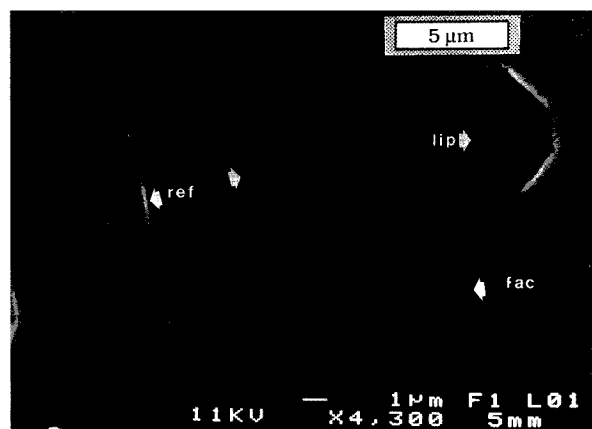
FIGURE 11. On the right, two tracks in \{11\bar{2}0\} (S type), showing the characteristic opening in the shape of an elongated hexagon with its long axis parallel to the crystallographic c axis. The upper track dips to the right and has a slightly inclined facet (lip) on the left-hand side of its opening. The lower track, which dips to the left, has a more steeply inclined facet (fac) on the opposite side. On the left, two residual etch figures (ref). Etching conditions: 300 s in 2.5% \text{HNO}_3 (set A).
