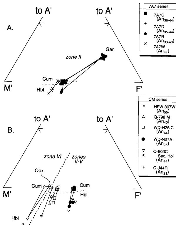
FIGURE 3. Ternary plot of the compositions of coexisting phases in samples from the (A) 7A7 series and (B) CM series. The diagram is a projection from plagioclase, quartz, and water. Coordinates: A' = \text{Al}_2\text{O}_3 + \text{Fe}_2\text{O}_3 + \text{TiO}_2 - \text{Na}_2\text{O} - \text{CaO} , M' = \text{MgO} , and F' = \text{FeO} + \text{MnO} - \text{TiO}_2 .
