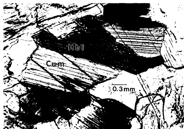
FIGURE 4. Photomicrograph of sample 7A7R that shows intergrown and extensive exsolution of clinoamphiboles. Coarsest visible lamellae are up to 2.5 μm thick.
