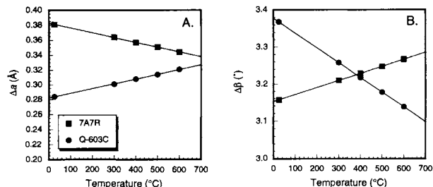
FIGURE 8. Variation of the differences in lattice parameters with temperature for cummingtonite and hornblende from samples 7A7R and Q-603C. (A) \Delta a = a_{\text{Hbl}} - a_{\text{Cum}} and (B) \Delta\beta = \beta_{\text{Hbl}} - \beta_{\text{Cum}} .
