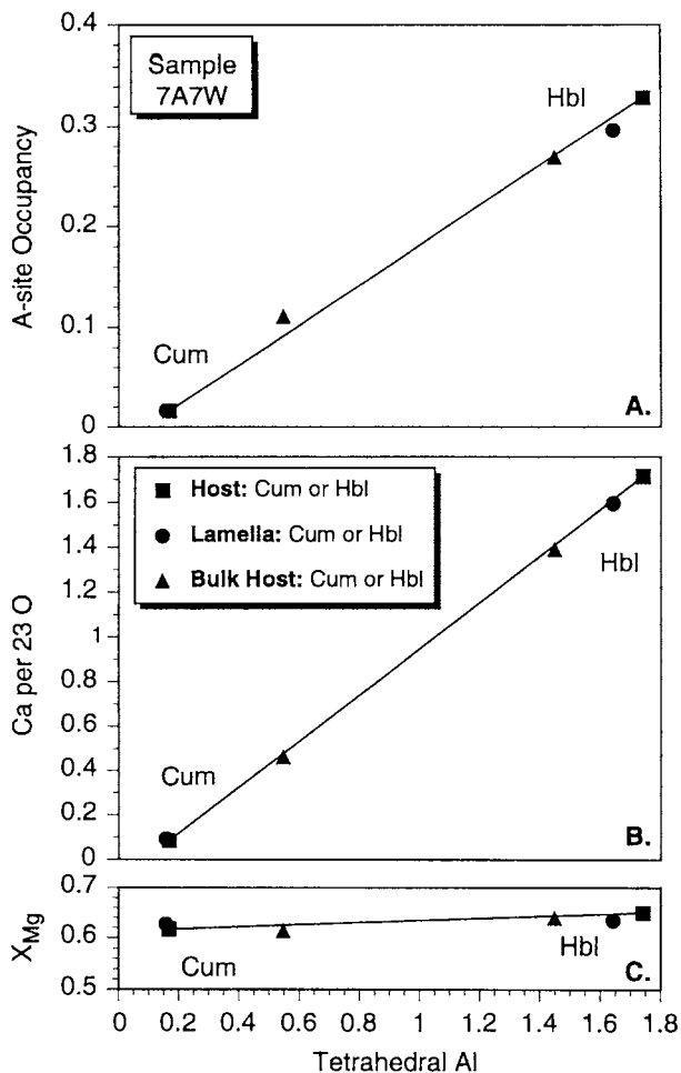
FIGURE 2. Three chemical plots of coexisting clin amphiboles (sample 7A7W). (A) ^{141}\text{Al} vs. A-site occupancy, (B) ^{141}\text{Al} vs. Ca per 23 O atoms, and (C) ^{141}\text{Al} vs. X_{\text{Mg}} . The bulk compositions of the host phases are averages of 60–70 electron microprobe point analyses across a single grain. Host and lamellar compositions were averages of 10–15 point analyses.
