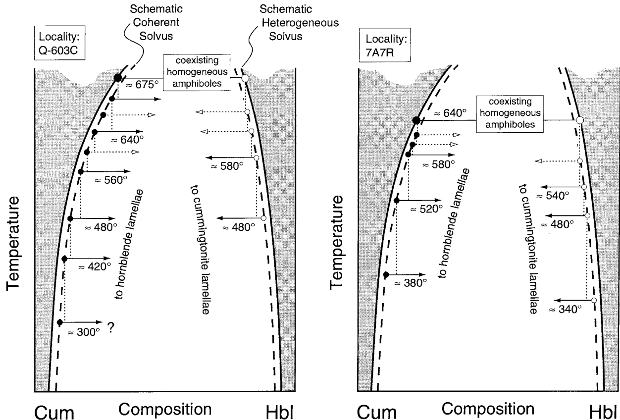
FIGURE 10. A schematic cummingtonite-hornblende solvus that summarizes the exsolution histories of samples Q-603C and 7A7R. Solid lines with arrowheads indicate that exsolution generation was characterized by both lamellar angle and average lamellar width; dashed lines with arrowheads indicate that the exsolution generation could only be characterized by average lamellar width (lamellar angle could not be measured). See text for discussion.
