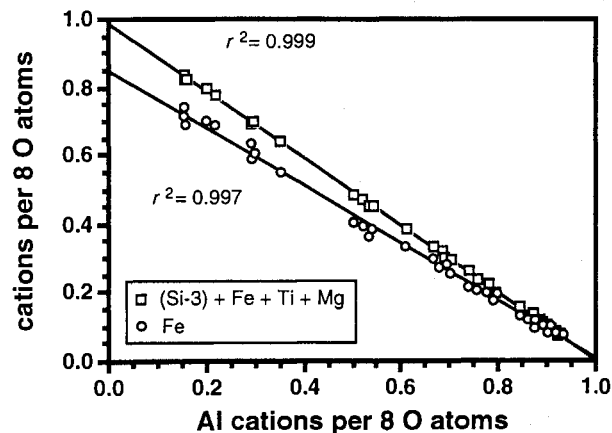
FIGURE 2. Cation plot of Al substitution in sanidine. Circles show that there is a progressive tetrahedral site deficiency for the exchange FeAl -1 . Only by including nonstoichiometric Si + Ti + Mg with Fe is the 1:1 substitution for Al preserved (squares).
