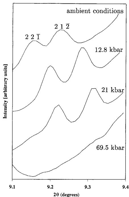
FIGURE 1. Evolution of 22\bar{1} and 21\bar{2} reflections with pressure. The slope in the background is due to the 031 reflection at 9.65^\circ 2\theta .
