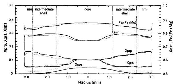
FIGURE 9. Garnet profiles for the most successful DiffGibbs model, shown with the measured profiles. The measured profiles from Figure 4 are shown as dotted lines, and the model profiles are shown as solid lines. Details of the correspondence of the measured and model profiles are discussed in the text.
