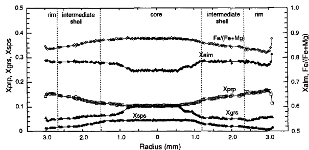
FIGURE 4. Profiles of mole-fraction almandine, pyrope, grossular, and spessartine components and \text{Fe}/(\text{Fe} + \text{Mg}) across the garnet shown in Figures 2 and 3. The line of the profile is shown in Figure 3. The profiles from left to right go from bottom to top of the image. Profiles were assembled from closely spaced quantitative spot analyses along a traverse of the garnet. Symbols along the profiles represent individual spot analyses. The curves were fit by eye to the analyses. Dotted vertical lines separate the profile into core, intermediate shell, and rim regions, which are also indicated in Figure 3.
