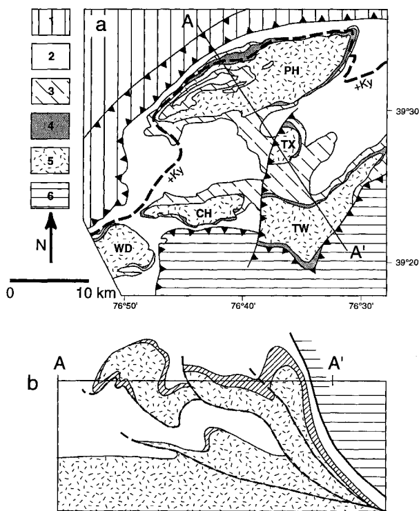
FIGURE 1. (a) Generalized geologic map of the eastern Maryland Piedmont (after Fisher 1989; Muller et al. 1989; Crowley et al. 1976). 1 = Low- to medium-grade metasediments of the western Piedmont; 2 = Loch Raven Formation, mainly pelitic schist; 3 = Cockeysville Marble; 4 = Setters Formation, quartzite and pelitic schist; 5 = Baltimore Gneiss, felsic basement gneiss; 6 = Baltimore Mafic Complex, island arc complex that collided with the Baltimore Gneiss terrane (units 2–5) during the Taconic Orogeny (at approximately 470 Ma). Anticlines in which the Baltimore Gneiss is exposed are labeled PH (Phoenix), TX (Texas), TW (Towson), CH (Chattolane), and WD (Woodstock). The line labeled A-A' shows the approximate location of the schematic cross section shown in b. (b) Schematic cross section A-A' through the Baltimore area after Fisher (1989). The random dash pattern represents the Baltimore Gneiss; the diagonal line pattern represents the Cockeysville and Setters Formations combined; the unpatterned area is the Loch Raven Formation, and the horizontal line pattern represents the Baltimore Mafic Complex. Bold dashed lines indicate thrust faults inferred by Fisher on the basis of the structural style of similar units in the Philadelphia area.
