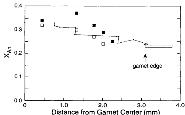
FIGURE 6. Graph of the composition of plagioclase inclusions vs. distance from the center of the garnet. The compositions shown are quantitative spot analyses of cores and rims of individual plagioclase inclusions. Cores of plagioclase inclusions are represented by solid squares, and rims are represented by open squares. The open bar beyond the garnet edge represents the average of spot analyses of matrix plagioclase rims. The line connecting small dots shows the composition of plagioclase calculated by the DiffGibbs model as a function of model-garnet radius.
