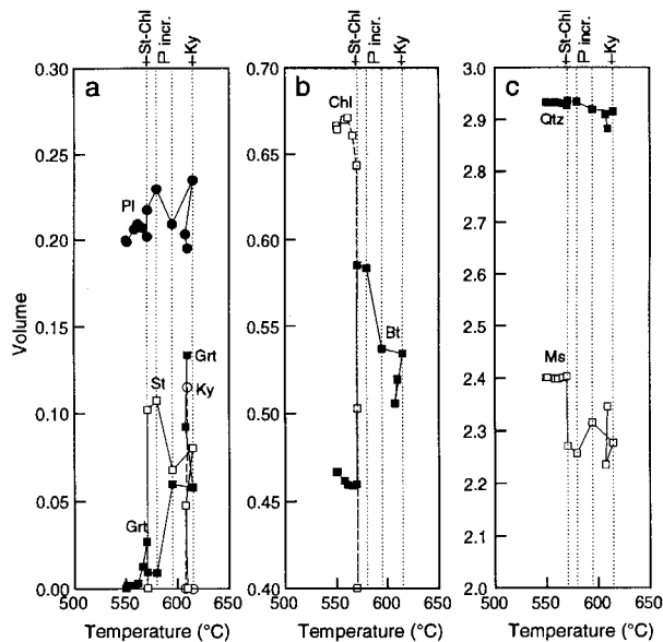
FIGURE 12. Calculated modes from the most successful model for all mineral phases included in the model as a function of temperature. The temperature at which staurolite was added and chlorite removed, the temperature range of the pressure increase, and the temperature at which kyanite was added are indicated by vertical dotted lines. (a) Abundances of garnet, staurolite, kyanite, and plagioclase; (b) abundances of biotite and chlorite; (c) abundances of muscovite and quartz.
