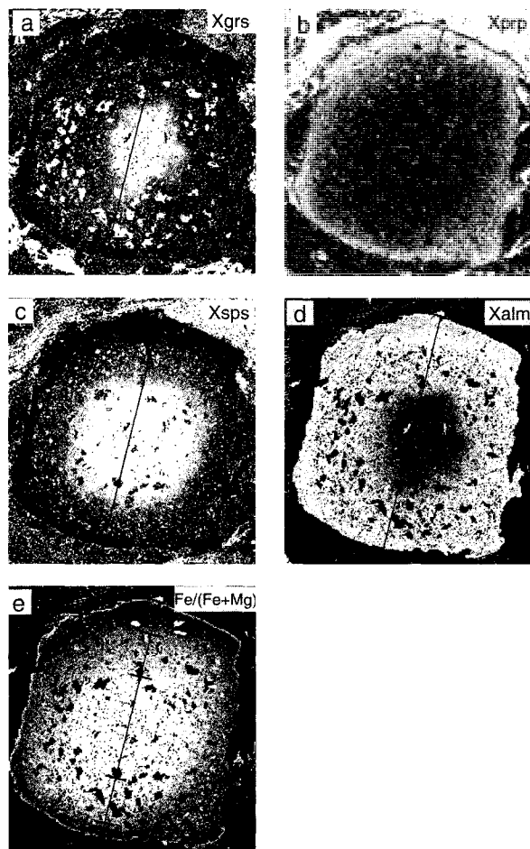
FIGURE 3. Gray scale maps of the mole fraction of components of the garnet shown in Figure 2b: (a) grossular, (b) pyrope, (c) spessartine, (d) almandine, and (e) Fe/(Fe + Mg). Bright areas have high concentration of a component, dark areas have low concentration. The gray scale on each map was adjusted separately to show the variation in concentration of that component. All images represent an area 6.5 mm wide by 6.9 mm high. The dark lines across the maps show the location of the profile along which the analyses shown in Figure 4 were taken. Line segments perpendicular to the line of the profile in e separate the garnet into core, intermediate shell, and rim regions that are referred to in the text.
