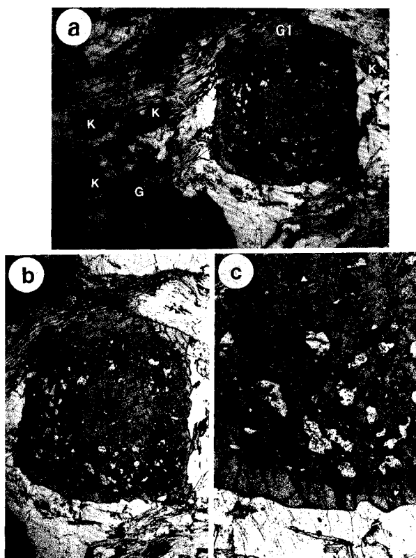
FIGURE 2. (a) Low-magnification photomicrograph of sample HV104, showing the relationship of the model garnet (G1) to the fabric and other phases in the sample. Staurolite (S with arrows, in lower right), kyanite (K), and another garnet (G) are labeled. The long dimension of the photomicrograph is approximately 13 mm. (b) Photomicrograph of the largest garnet in sample HV104, which is the basis for the modeling. Note the core, the intermediate plagioclase inclusion-rich region, and the inclusion-free rim of the garnet. The long dimension of the photomicrograph is approximately 10 mm. (c) A higher magnification photomicrograph of the lower, middle part of the garnet shown in b . The photograph shows the intermediate region of the garnet, which contains abundant plagioclase inclusions (bright, low-relief areas), and a portion of the inclusion-free rim. Note the faceted, negative garnet crystal shape of some of the inclusions and the dusty appearance produced by abundant small inclusions. The long dimension of the photomicrograph is approximately 3 mm. Maps of the anorthite content in plagioclase and the grossular content in garnet of the central portion of this area are shown in Figure 5.
