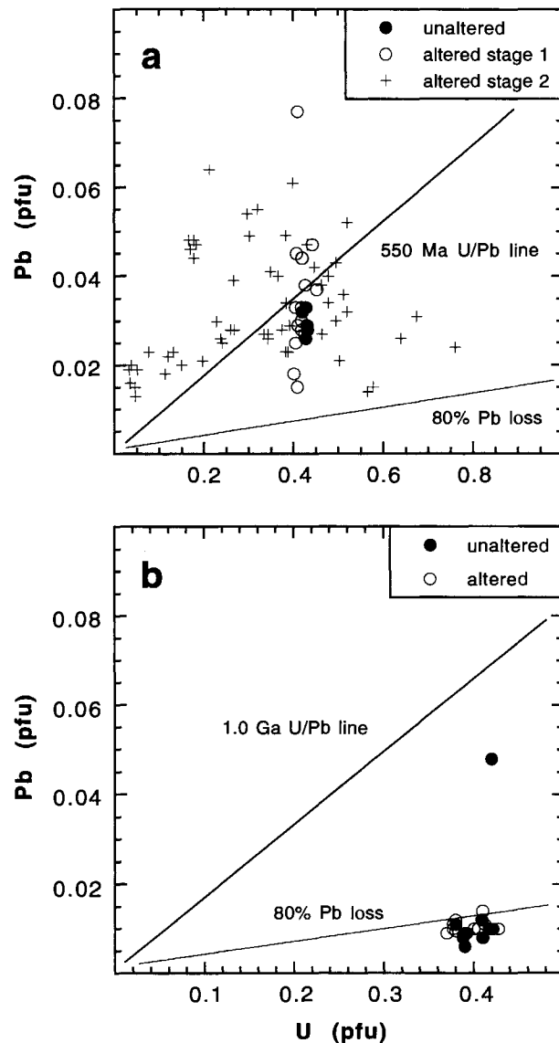
FIGURE 6. U-Pb systematics (atoms per formula unit) of unaltered and altered betafite samples. (a) Results for 550 m.y. old Madagascar samples 081, 155, 176, 205, and 210. (b) Results for 1000 m.y. old Canadian samples 083 and 204. A single high Pb data point may have resulted from a small grain of galena located within the excitation volume of the electron probe.
