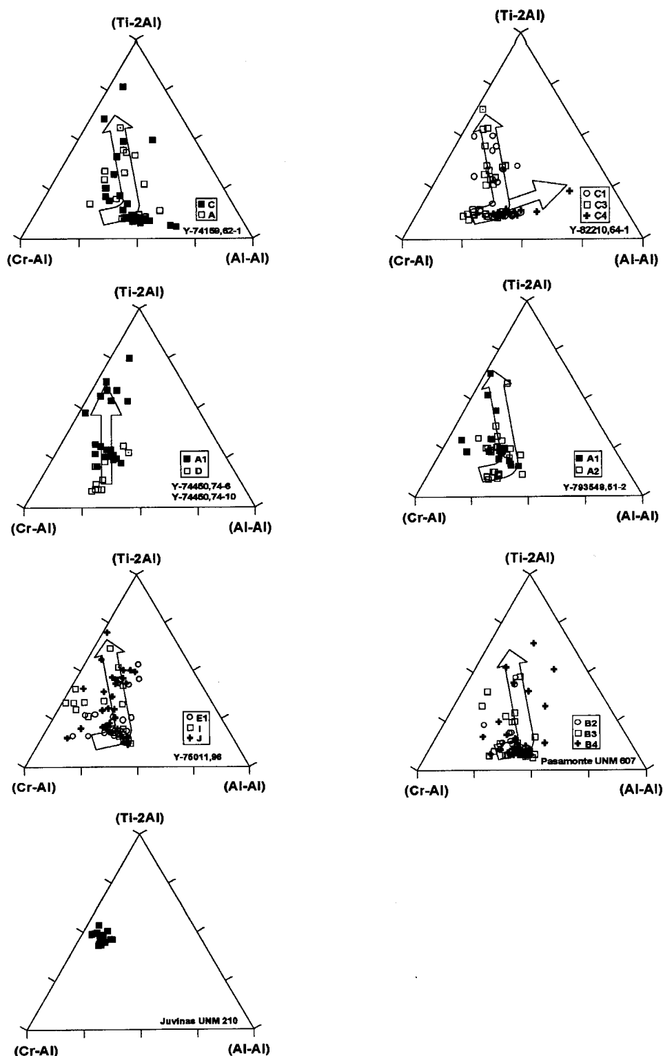
FIGURE 6. Ternary plots of the three types of substitutional couples ( ^{16}\text{Cr}^{3+}-^{14}\text{Al}^{3+} , ^{16}\text{Al}^{3+}-^{14}\text{Al}^{3+} , and ^{16}\text{Ti}^{4+}-2^{14}\text{Al}^{3+} ) for each of the grains analyzed. The average grain compositions from Juvinas UNM 210 are shown for comparison with grains that are composed of fine intergrowths of two pyroxenes and oxides. Arrows indicate direction of crystallization from core to rim. All the arrows are similar except for Y-82210 C4, indicating pyroxene crystallization without the onset of plagioclase crystallization, and Y-74450 D primarily represents the core of the grain and therefore dominantly reflects the initial ^{16}\text{Cr}^{3+}-^{14}\text{Al}^{3+} couple.
