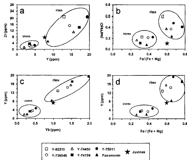
FIGURE 8. (a) Zr vs. Y from averaged analyses. A positive correlation was observed between the two elements. (b) (\text{Nd/Yb})_{\text{Cl}} (normalized) vs. \text{Fe}/(\text{Fe} + \text{Mg}) from averaged analyses. Note that all the core-rim pairs increase in (\text{Nd/Yb})_{\text{Cl}} with increasing \text{Fe}/(\text{Fe} + \text{Mg}) . (c) Y vs. Yb from averaged analyses. The positive correlation is a result of the geochemical similarities of the two elements. (d) Y vs. \text{Fe}/(\text{Fe} + \text{Mg}) from averaged analyses.
