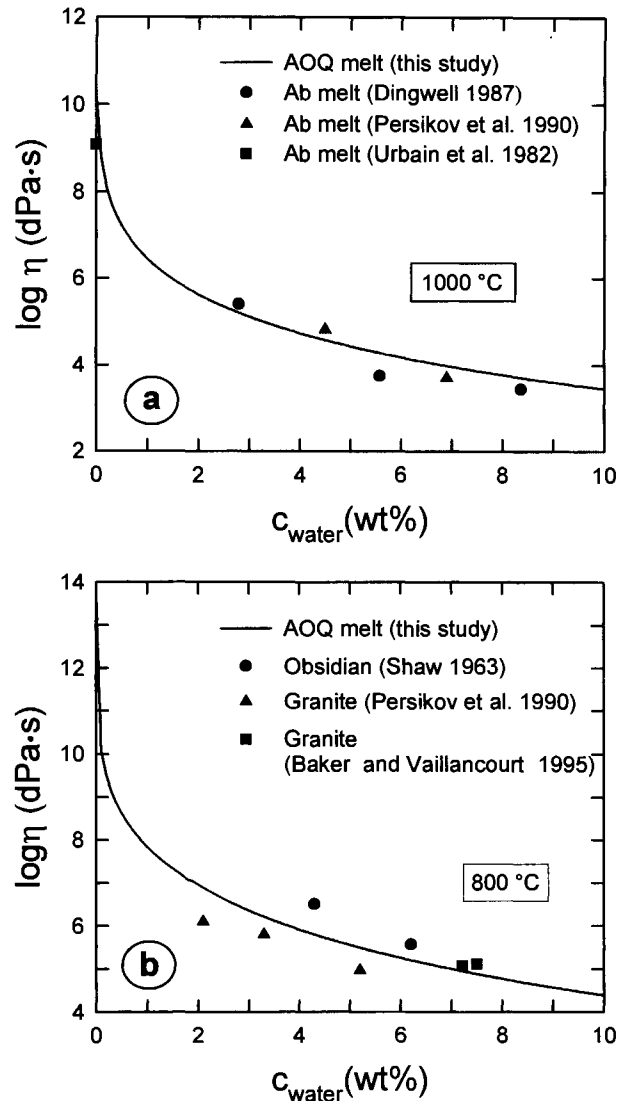
FIGURE 7. (a) Comparison between the viscosities of AOQ melts (curve) and the viscosities of albite melts as a function of H 2 O content at a temperature of 1000 °C. Viscosities taken from Dingwell (1987) were measured at 7.5 kbar, from Persikov et al. (1990) at 2 and 6 kbar, and from Urbain et al. (1982) at 1 bar. (b) Comparison between the viscosities of AOQ melts (curve) and the viscosities of natural granitic melts as a function of H 2 O content at a temperature of 800 °C. Viscosities taken from Baker and Vaillancourt (1995) were measured at 10 kbar, from Persikov et al. (1990) at 0.5, 1, and 2 kbar, and from Shaw (1963) at 1 and 2 kbar. H 2 O content for granitic melts from Baker and Vaillancourt (1995) was taken as the sum of H 2 O and F in the melt [see Baker and Vaillancourt (1995) for details].
