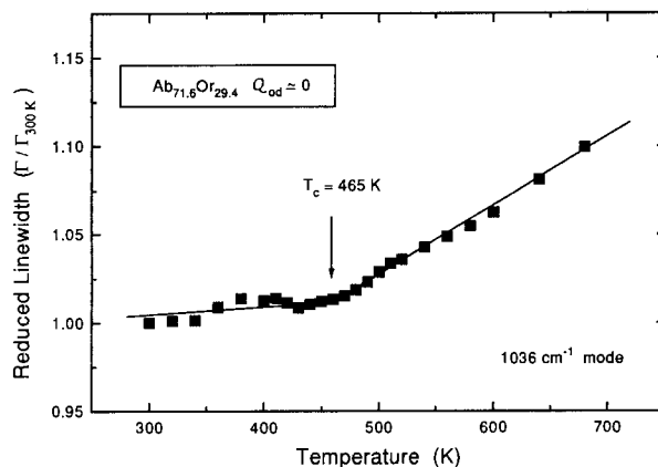
FIGURE 13. The change in the temperature dependence of the reduced line width of the 1036\text{ cm}^{-1} mode in \text{Ab}_{71.6}\text{Or}_{29.4} ( Q_{od} = 0 ) at 465\text{ K} corresponds to the structural phase transition C2/m-C\bar{1} .
