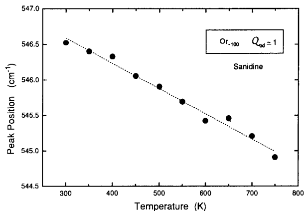
FIGURE 11. Temperature dependence of the 535\text{ cm}^{-1} phonon in sanidine ( \text{Or}_{100} , Q_{od} \approx 1 ).
