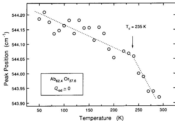
FIGURE 12. Thermal frequency shift of the 544\text{ cm}^{-1} phonon with a structural phase transition C2/m-C\bar{1} at T_c = 235\text{ K} ( \text{Ab}_{62.4}\text{Or}_{37.6} , Q_{od} = 0 ).
