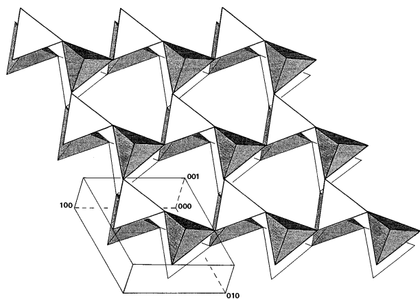
FIGURE 1. Crystal structure of kalsilite with P31c symmetry showing tetrahedral layers perpendicular to c . Shaded and empty tetrahedra represent T1 and T2, respectively. K atoms are not shown.
