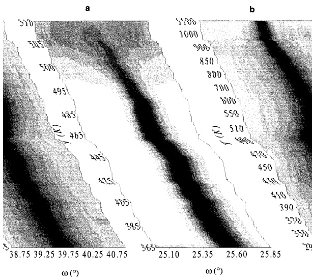
FIGURE 2. Temperature evolution of the rocking-curve profiles of reflections \bar{2}16 (a) and \bar{1}42 (b).
