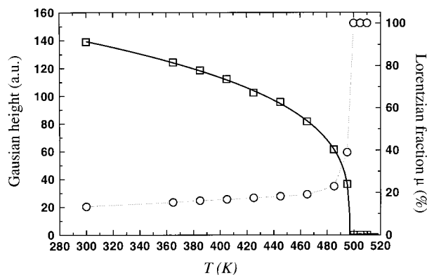
FIGURE 3. Temperature dependence of the Gaussian heights (squares) and Lorentzian fractions \mu (circles) of reflection \bar{2}16 . The solid line is the fit to the heights ( \propto Q^2 ) yielding \beta = 0.146(3) and T_c = 497.0(4) K.
