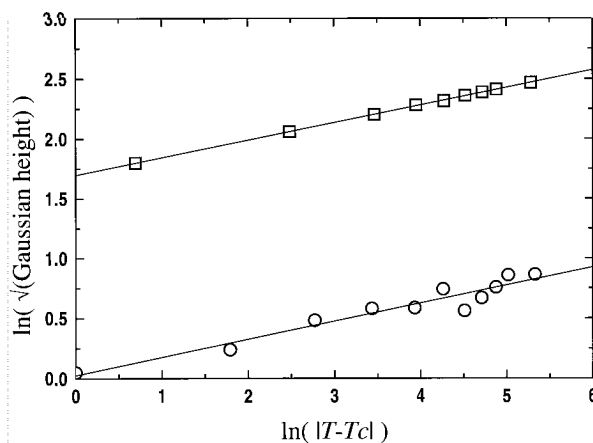
FIGURE 4. Double logarithmic plot of the square root of the Bragg intensity (Gaussian component) vs. the reduced temperature |T - T_c| of reflections \bar{2}16 (squares) and \bar{1}43 (circles). The solid lines are linear fits to the data; the slope is the order parameter exponent \beta .
