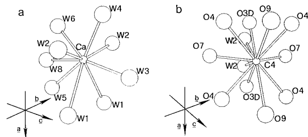
FIGURE 5. Change of the Ca atom coordination during dehydration. (a) Ca- \text{H}_2\text{O} molecule coordination (distances < 2.75 \text{ \AA} ) in stilbite A at 315 K; (b) C4-framework O atoms and \text{H}_2\text{O} molecule coordination (distances < 3.10 \text{ \AA} ) in stilbite B at 521 K.
