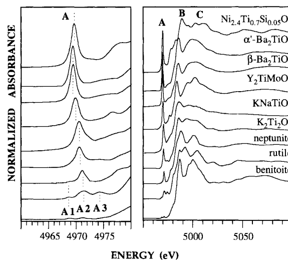
FIGURE 1. (right) Normalized Ti K -edge XANES spectra for selected Ti-bearing model compounds containing 141 Ti, 151 Ti, and 161 Ti. (left) Detail of the normalized preedge feature.
