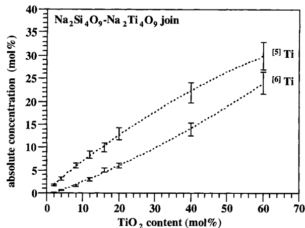
FIGURE 6. Plot of the absolute molar concentrations calculated for 5 Ti and 6 Ti (based on preedge models listed in Table 3) for the NTS glasses. Note the rapid increase of 6 Ti at high TiO 2 contents.
