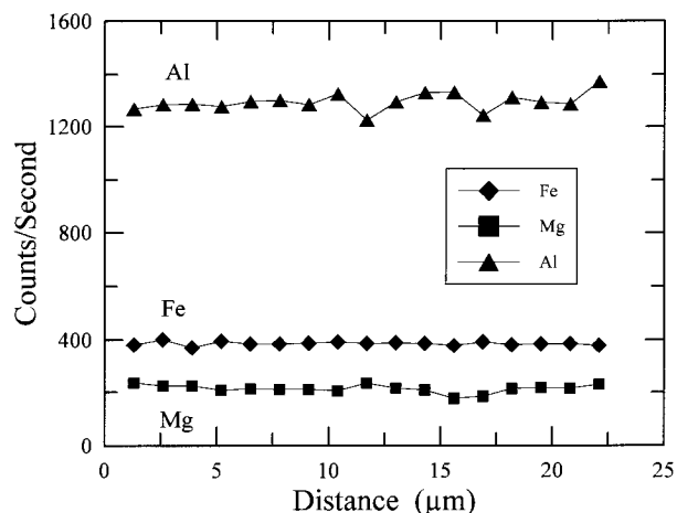
FIGURE 1. Element concentration profile across a 24 \mu\text{m} wide garnet crystal ( \text{Alm}_{30}\text{Py}_{20} ), synthesized at 900 ^{\circ}\text{C} and 1.5 GPa.
