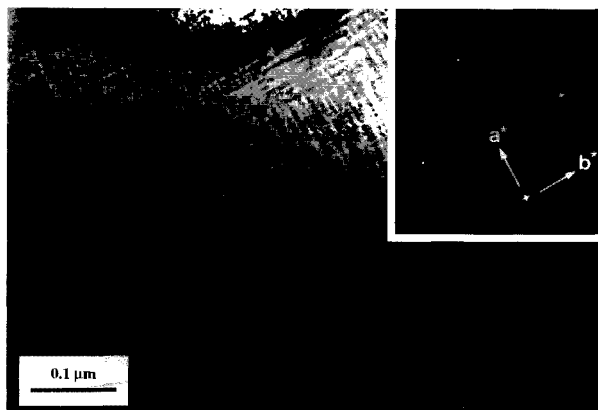
FIGURE 1. Bright-field electron micrograph of sample e24, showing compositional modulations developed parallel to \{100\} . Inset is the selected-area diffraction pattern of sample e24 recorded with the electron beam parallel to [001] . Diffraction spots have a distinctive cross shape, which is characteristic of tweed-textures produced by spinodal decomposition.
