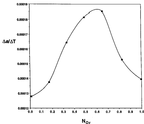
FIGURE 2. Slope of the a unit-cell dimension with temperature from Figure 1 plotted as a function of mole fraction \text{KAISi}_3\text{O}_8 ( N_{\text{Or}} ). The curve is interpolated and is not a least-squares fit.
