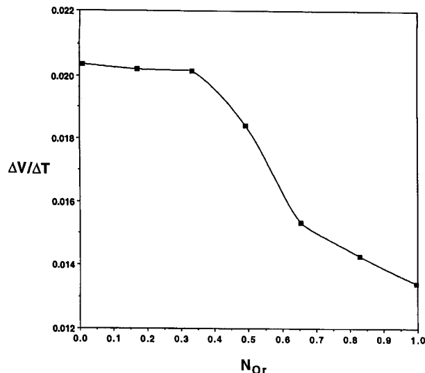
FIGURE 6. Slope of unit-cell volume as a function of temperature from Figure 5 plotted against composition. Note that the slope is high for the three most sodic feldspars, then falls off steeply with increasing K content.
