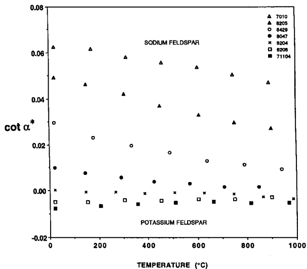
FIGURE 4. Plot of \cot \alpha^* vs. temperature for all feldspars. Values for potassic feldspars are bunched and essentially constant with temperature. Sodic feldspars become more widely spaced, and values decrease with temperature.
