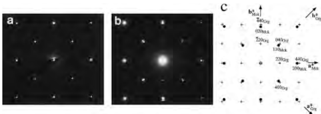
FIGURE 4. (a) Electron diffraction pattern obtained from mackinawite parallel to (001) before heating. The space group of mackinawite is P4/nmm . The n -glide plane parallel to (001) results in the systematic absence of hk0 reflections for which h + k \neq 2n (where n is an integer). (b) Electron diffraction pattern from mackinawite parallel to (001) after heating to 473 K, showing extra
