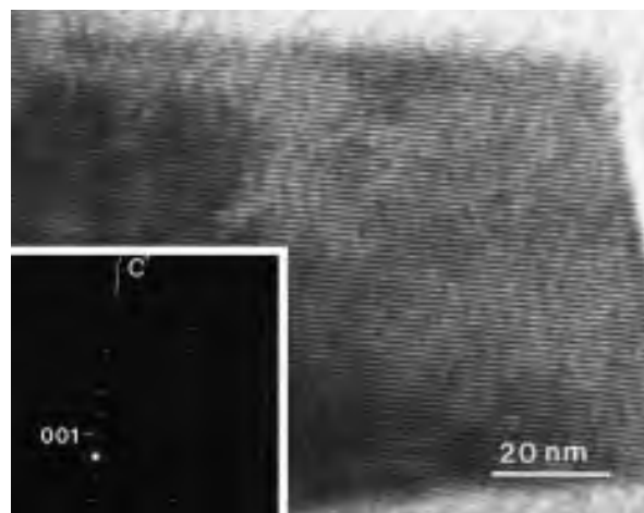
FIGURE 4. Lattice-fringe image of well-ordered ferroceladonite. The inset electron diffraction pattern shows sharp 0kl reflections consistent with the 1M polytype.
