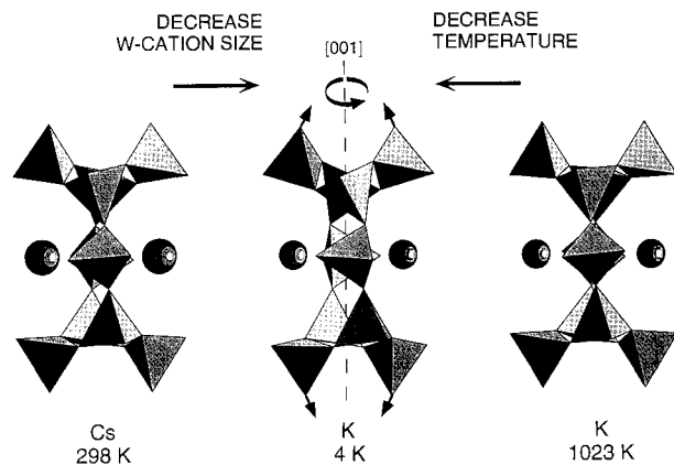
FIGURE 9. Distortion of the leucite structure induced by temperature or composition. The structure may be visualized in terms of tetragonal prisms with their long axes parallel to [001] . The view direction is [110] . The channel-cation sites, depicted as spheres, are connected by side channels passing through eightfold tetrahedral rings. Smaller channel cations (e.g., K replacing Cs), or reduced temperatures, induce a twisting distortion in the prisms (the upper ring rotates around [001] , relative to the lower ring). This causes axial elongation, but radial compression. Metrically, c is extended, whereas a and b are decreased.
