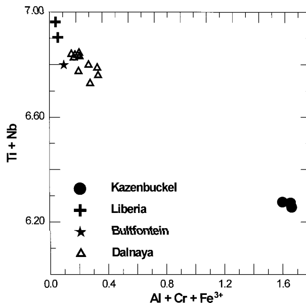
FIGURE 6. Plot of freudenbergite Σ B 3+ vs. Ti and Nb from all known localities. Solid circles are those from Katzenbuckel (McKie and Long 1970; Frenzel et al. 1971) crosses are Liberian (Haggerty 1983), stars are from Bultfontein (Haggerty 1989), and triangles are from Dalnaya (this study).
