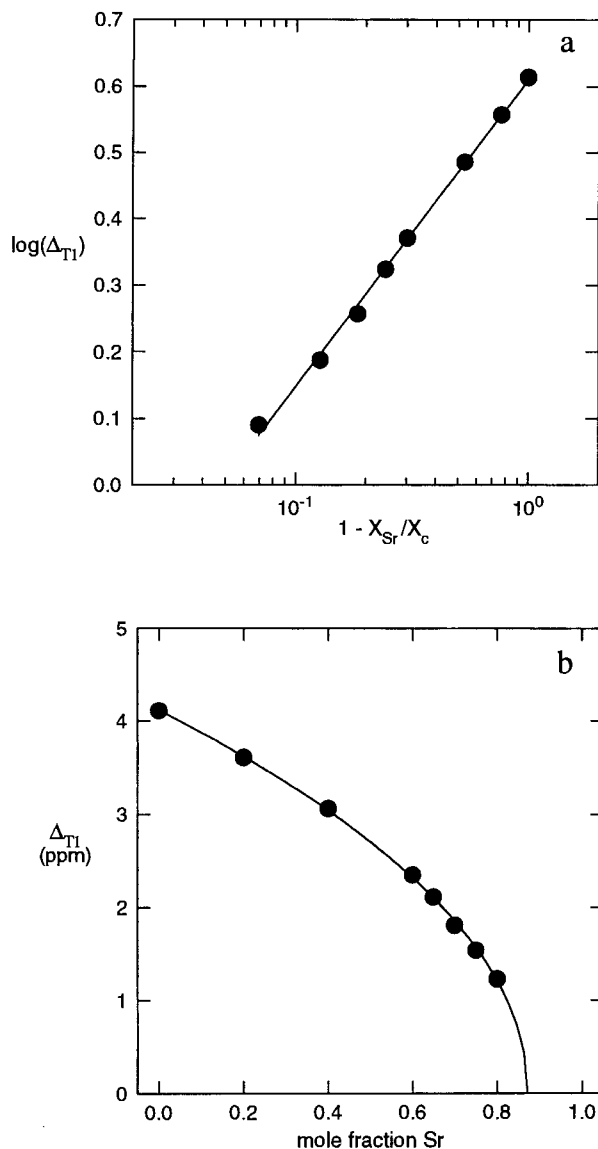
FIGURE 4. Composition dependence of the difference in ^{29}\text{Si} NMR chemical shift ( \Delta_{T1} ) between the peak assigned to T1mz for \bar{1} samples and that assigned to T1o in the I2/c phase. (a) Log-log plot with reduced composition; critical composition X_c = 0.86 taken from XRD results (McGuinn and Redfern 1994). Linear relationship indicates \Delta_{T1} \propto Q (Eq. 4), and its slope corresponds to critical exponent, \beta = 0.46 . (b) Line is a least-squares fit to Equations 4 and 5, giving \beta = 0.49(2) and X_c = 0.87(3) .
