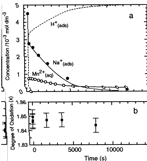
FIGURE 1. (a) Temporal behavior of H^+ (ads), Na^+ (ads), and Mn^{2+} (aq) for NaBu undergoing structural alteration at pH 4. The solid line shown for Mn^{2+} (aq) is an interpolation of the experimental data, whereas the line shown for Na^+ (ads) was calculated on the basis of charge balance considerations, assuming only Na^+ , H^+ , and Mn^{2+} in the exchange process. Total Mn concentration is 1.54 \times 10^{-2} \text{ mol/dm}^3 . (b) Degree of oxidation ( x in MnO_x ) for NaBu undergoing structural alteration at pH 4.
