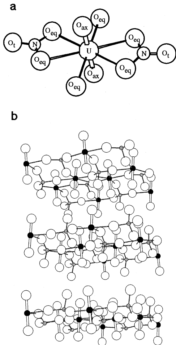
FIGURE 1. (a) Basic structural unit of uranyl nitrate. Different O atom environments are distinguished by axial ( O_{ax} ), equatorial ( O_{eq} ), and terminal ( O_t ) designations. Equatorial O atoms that are not bonded to N are part of H_2O molecules. (b) Extended layer structure of \alpha -uranophane. Solid circle, represents U atoms, Shaded are Si, and open are O. Basic units similar to that shown in (a) are bonded together through U-O_{eq}-Si-O_{eq}-U linkages in uranophane. Linear uranyl moieties are approximately perpendicular to layers.
