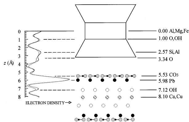
FIGURE 7. One-dimensional curves of electron density as a function of z values from 00l diffraction intensities of surite. Solid line: calculated. Dotted line: observed. The corresponding structural model is shown.
