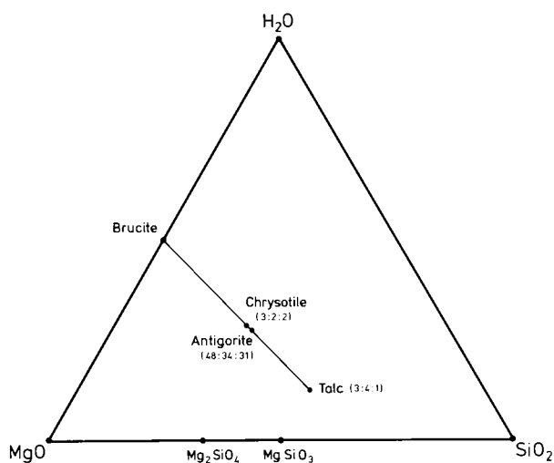
FIGURE 1. Selected phases in the system MgO - SiO_2 - H_2O (MSH). The molar ratios of MgO:SiO_2:H_2O are given in parentheses. Solid line emphasizes the colinearity of compositions of brucite, chrysotile, antigorite, and talc.
