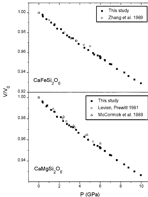
FIGURE 2. Pressure dependence of the unit-cell volumes for diopside and hedenbergite
