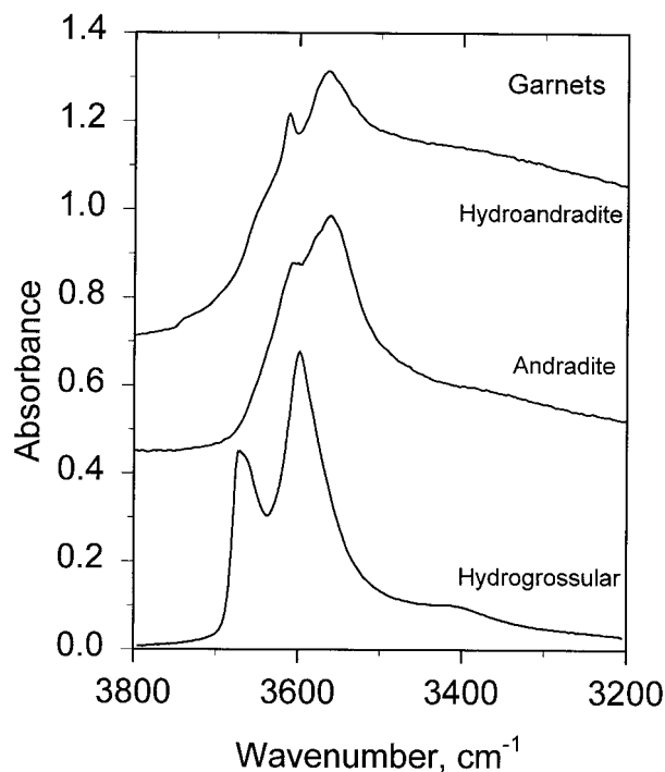
FIGURE 2. Comparison of the IR spectra of hydrogrossular from Crestmore, California, Ca 3 Al 2 [(SiO 4 ) 1.64 (O 4 H 4 ) 1.36 ] (Rossman and Aines 1991); hydrous andradite from Bombay, India (GRR1669); synthetic hydroandradite Ca 3 Fe 3+ [(SiO 4 ) 2.81 (O 4 H 4 ) 0.19 ] (GAIV1/4). The spectra are scaled for comparable band heights, i.e., 4.2 μm thickness (Crestmore); 10.5 μm thickness (Bombay); and powdered synthetic hydroandradite.
