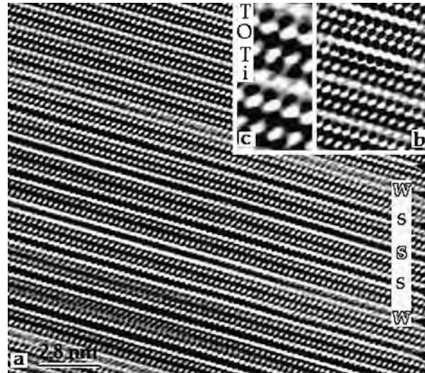
FIGURE 6. (a) Rotationally filtered Scherzer defocus [010] image of partially altered chlorite (bottom) and associated 1.0 nm phase. Arrows indicate brucite-like interlayers with variable S (strong) vs. W (weak) contrast. To our knowledge, [010] zone axis atomic-resolution images of layer silicates have not been previously published. Consequently, the area in (b) is enlarged (with superimposed image simulation) and in (c) is labeled to show the correspondence between tetrahedral cations (spots), the octahedral sheet (spotty stripes) and the interlayer. Simulations and details for chlorite are shown elsewhere.
