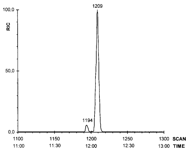
FIGURE 1. Gas chromatogram of original hartite crystals indicating high chemical purity of the material studied. The smaller peak at scan 1194 corresponds to an admixture that is 4.31% of the total weight amount.
