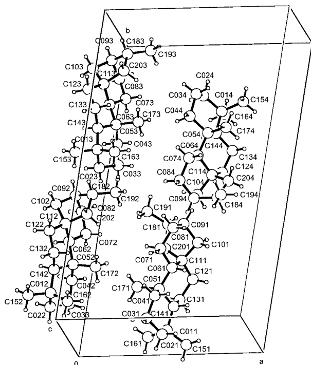
FIGURE 4. View of the unit cell of hartite with atom labeling. Note four symmetrically independent molecules similar to each other.
