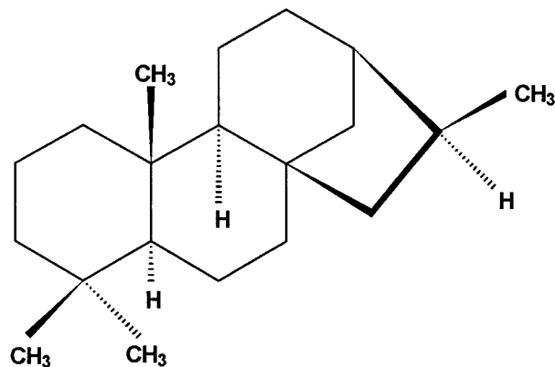
FIGURE 3. Stereochemical structure of (+)-phyllocladane, i.e., the basic unit of hartite. Thick lines are under the plane; dotted lines are below the plane.
