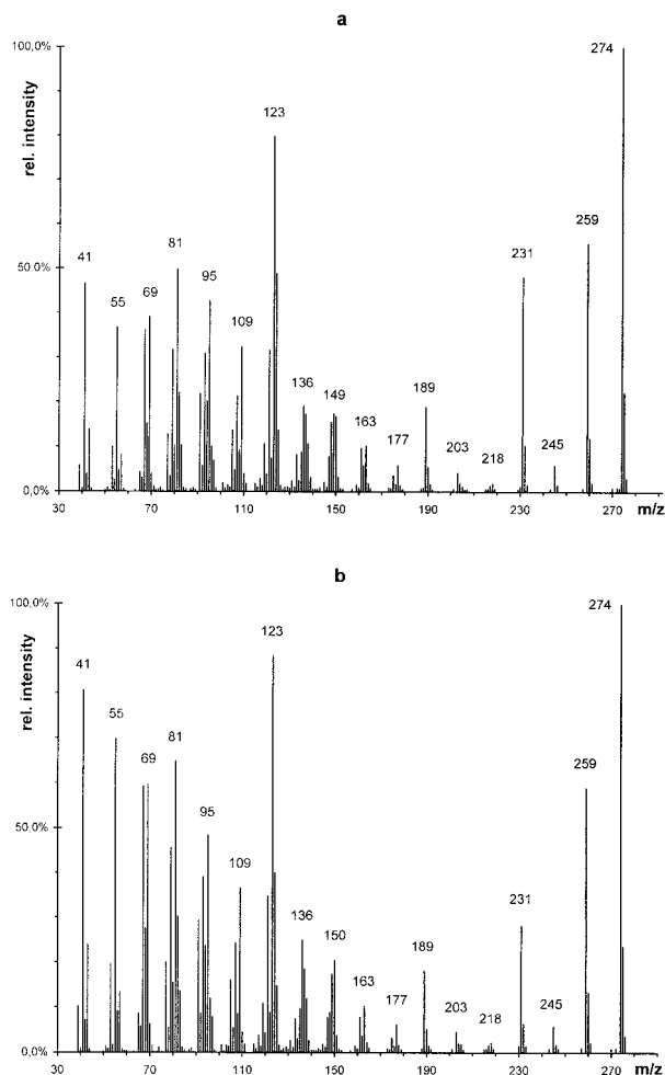
FIGURE 2. Mass spectra of (a) the smaller peak at scan 1194 [probably (-)-phyllocladane] and (b) the major component, i.e., (+)-phyllocladane.
