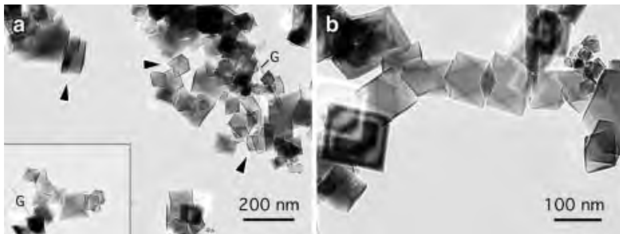
FIGURE 7. Low-magnification TEM micrographs of synthetic magnetite. (a) Typical aggregates showing slightly distorted octahedral morphologies, the wide range of sizes, and a few twinned crystals (arrowed). The needle-shaped crystals (G) are goethite. (b) A small chain of octahedra, some of which share {111} faces.
