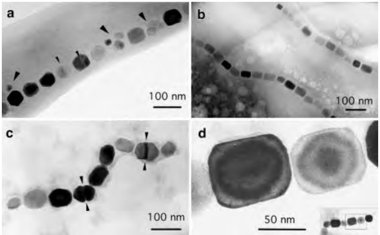
FIGURE 1. Low-magnification TEM micrographs of chains of magnetosomes, showing various morphologies. (a) Cubooctahedral crystals, twinned crystals (small arrows), and clusters of small crystals (large arrows) in M. magnetotacticum . (b) Rectangular crystals in strain MV-1. (c) Elongated crystals, some with re-entrant angles characteristic of twinning (arrowed), in strain MV-4; (d) Rectangular crystals with thickness fringes in strain MC-1.
