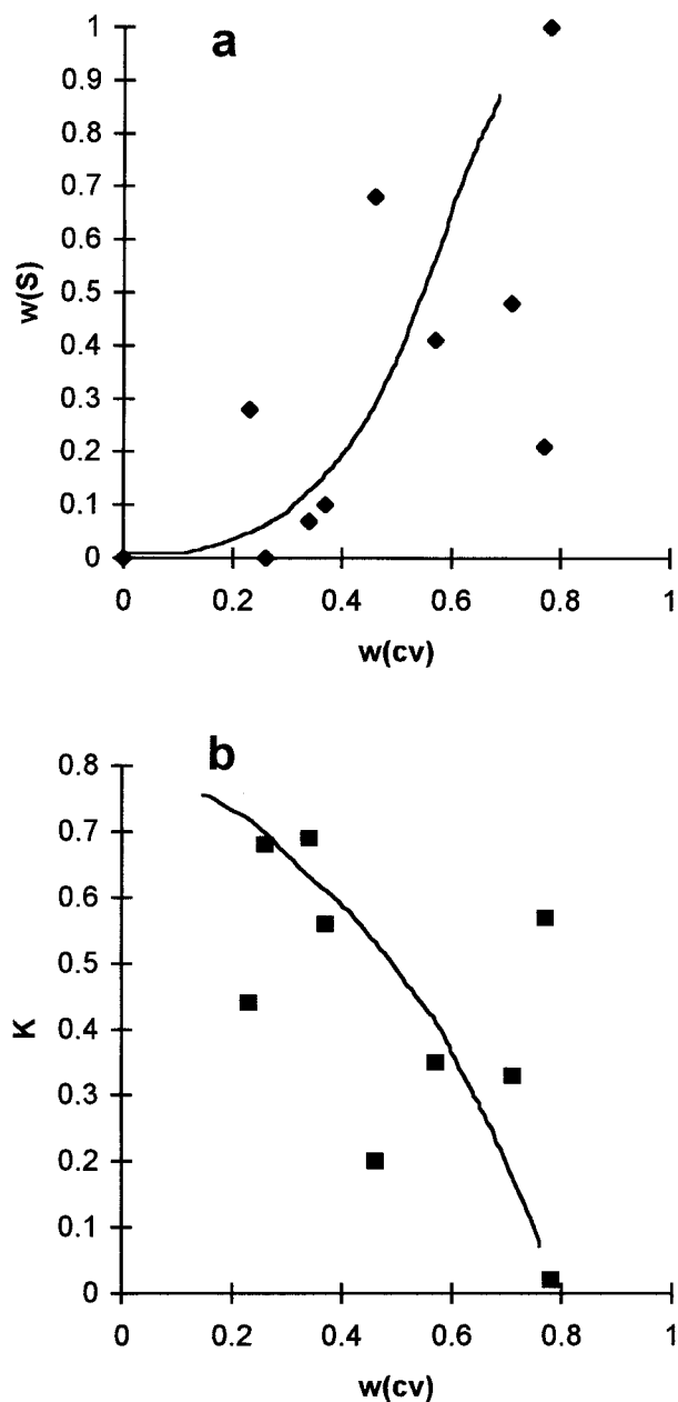
FIGURE 9. The dependence between w_{cv} determined by EWA and w_s (a) and the content of fixed K per O_{10}(OH)_2 (b).
