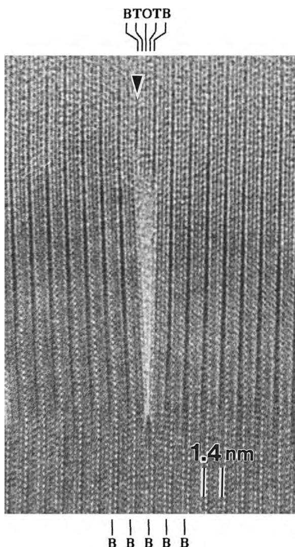
FIGURE 6. A single triangular region observed from \langle 100 \rangle . B, T, and O indicate the position of brucite-like interlayer, tetrahedral and octahedral sheet in TOT layer, respectively. Note one TOT layer and two brucite-like sheets are missing at the top of the triangle. The arrowhead indicates the brucite-like sheet which is first terminated compared with another brucite-like sheet and the TOT layer. One the other hand, no brucite-like interlayer is missing where the triangle is closed at the bottom of the figure.
