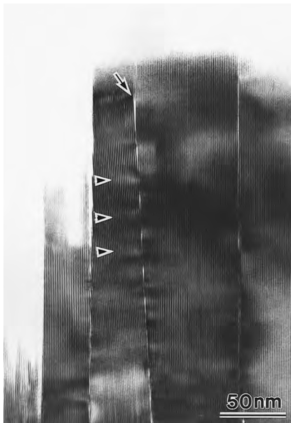
FIGURE 3. HRTEM image of chlorite in a chlorite-quartz-chalcopyrite vein. The beam direction is \langle 010 \rangle . The arrow indicates the point where a LAGB is initiated.
