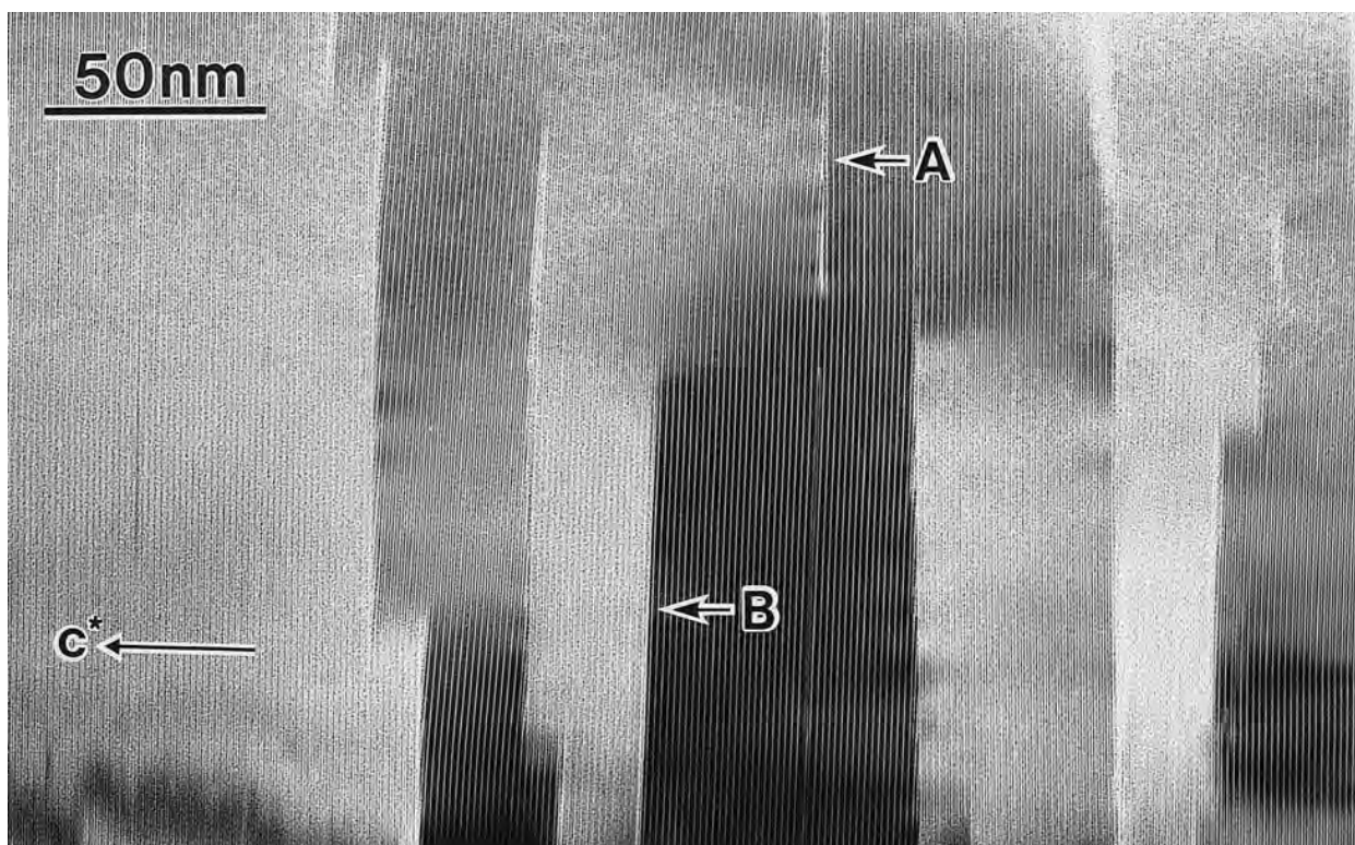
FIGURE 1. HRTEM image of chlorite from altered granite observed approximately along \langle 010 \rangle . Planar defects are observed commonly as indicated by the arrows A and B. At defect A the lattice fringes are inclined to each other whereas at defect B (001) fringes are almost parallel on both sides of the defect. Some planar defects are initiated or terminated in the grain.
