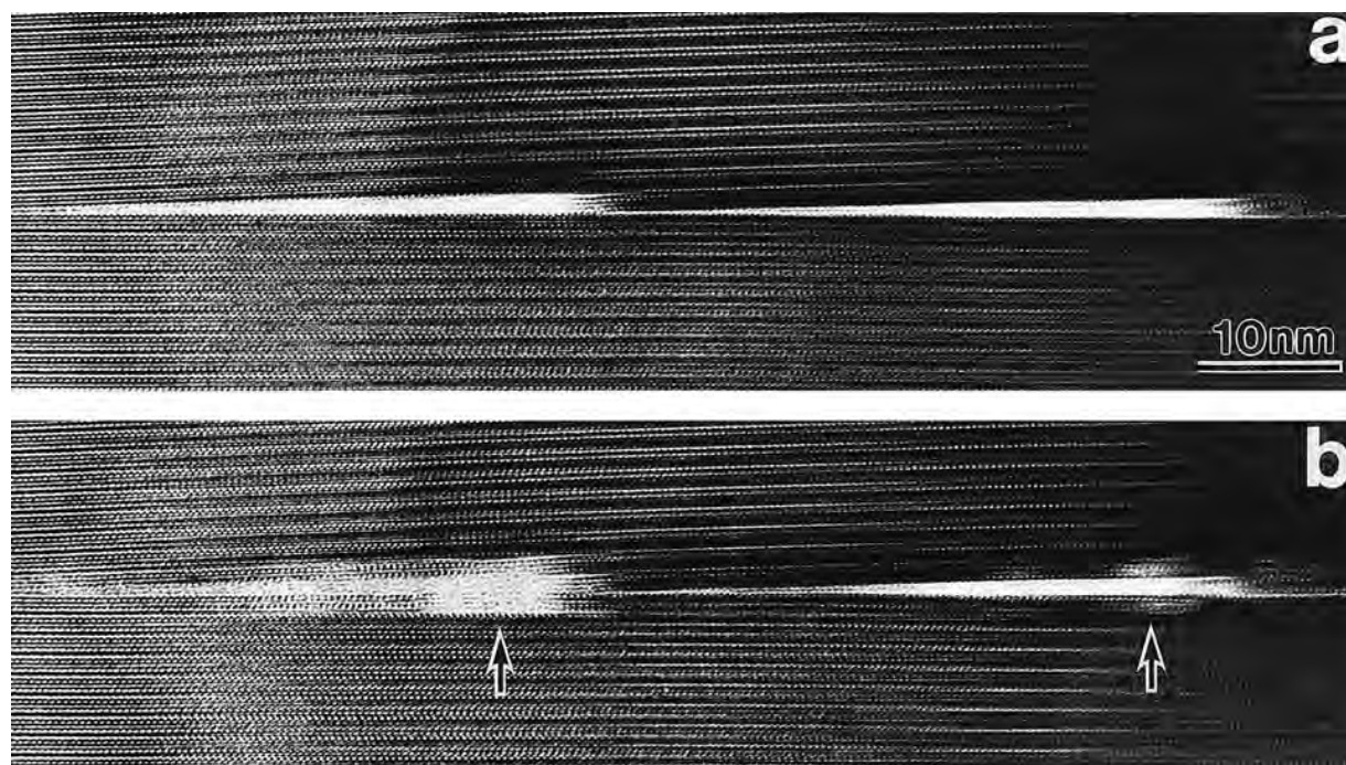
FIGURE 5. (a) Magnified image of a LAGB observed from \langle 100 \rangle . (b) Image of the same area after beam radiation for about 20 s. The chlorite layers on both sides of the boundary are starting to be vitrified as indicated by arrows. The structure in the chlorite layer can be distinguished in the thinner area (left side).
