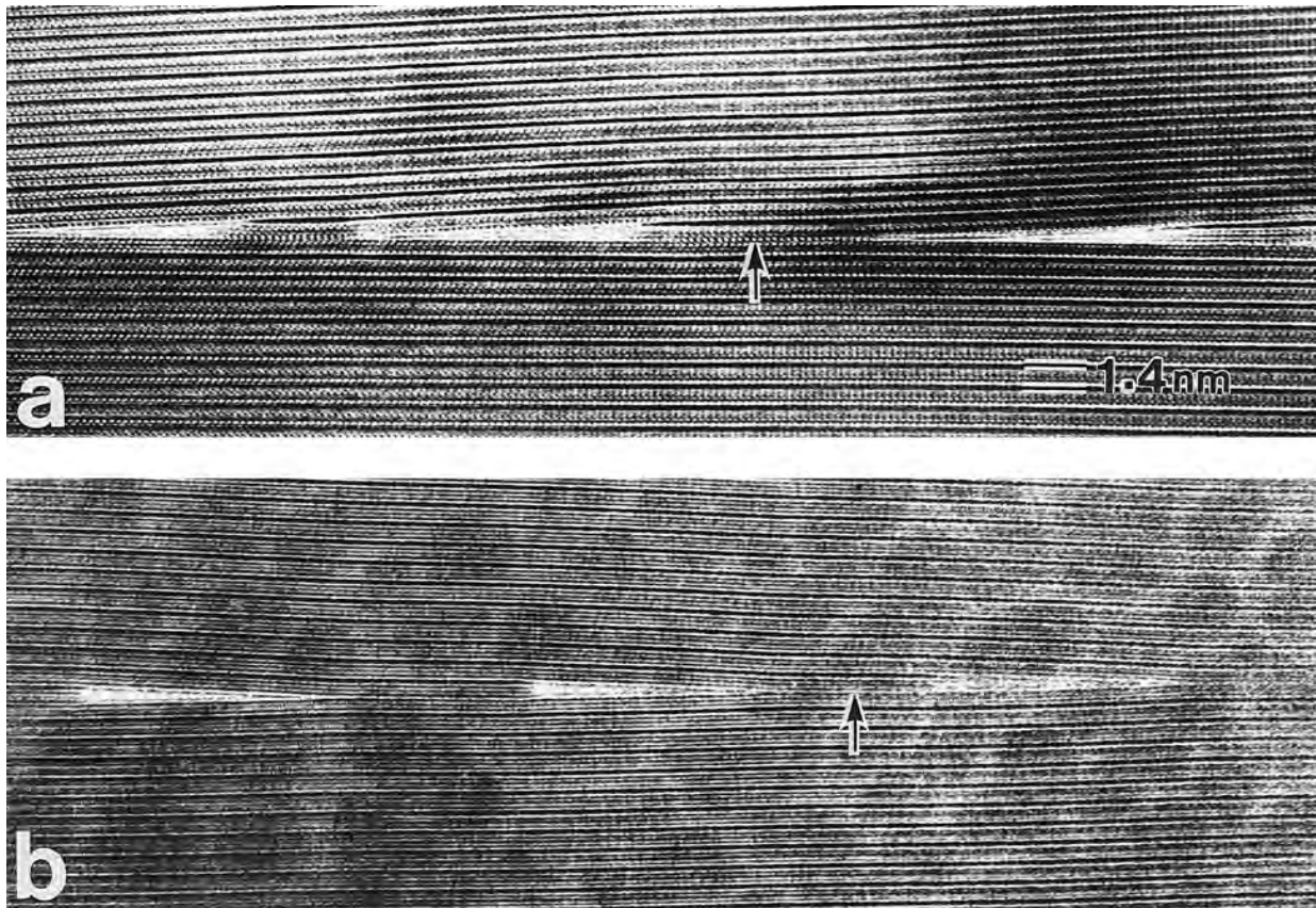
FIGURE 4. (a) Magnified image of a LAGB whose common axis is \langle 100 \rangle . The terminating chlorite layers are bent in contact with the layer on the other side of the boundary (view the photograph at a low angle along the boundary). (b) Magnified image of another LAGB whose common axis is \langle 010 \rangle . Three cation sheets in a TOT layer correspond to three fine black lines and the brucite-like layer has the contrast of the boldest black line. It is clearly indicated that two TOT layers are in contact without a brucite-like sheet at the area indicated by the arrow in both figures.
