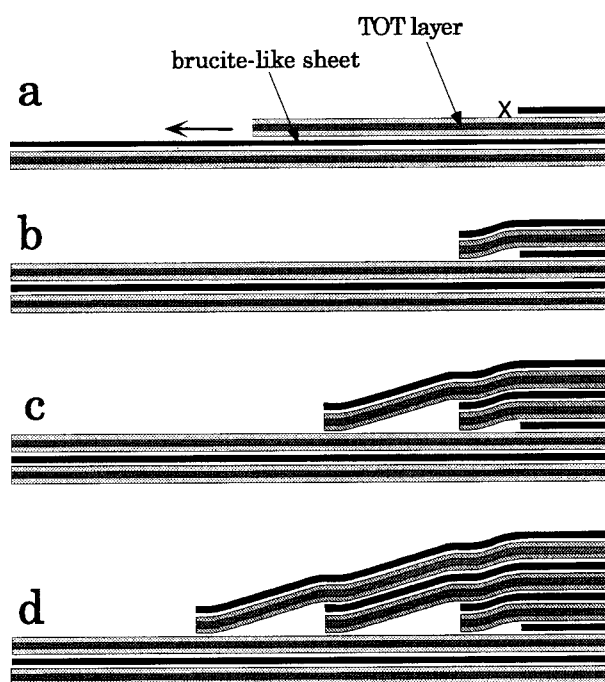
FIGURE 7. Schematic illustration of the formation mechanism of LAGB (see text for details).
