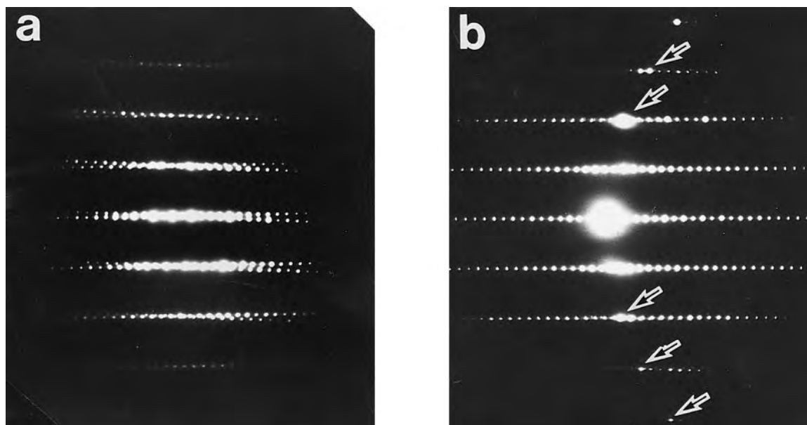
FIGURE 2. SAED pattern from areas that contains planar defects similar to (a) defect A or (b) defect B in Figure 1. The beam direction is \langle 010 \rangle . Both c^* axes are on the observing plane in a whereas one is on the plane and the other is not, but forming an arc of zero-order Laue zone (ZOLZ) as indicated by arrows in b .
