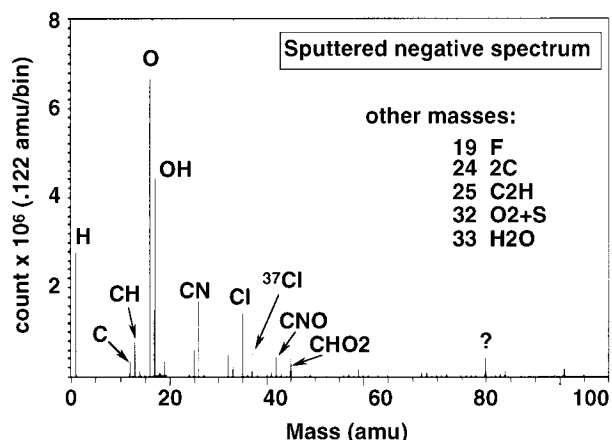
FIGURE 2. Negative mass spectrum corresponding to the positive spectra of Figure 1. Note that this is from the sputtered surface. The spectrum was collected for 30 min. Mass peaks are listed in Table. 1
