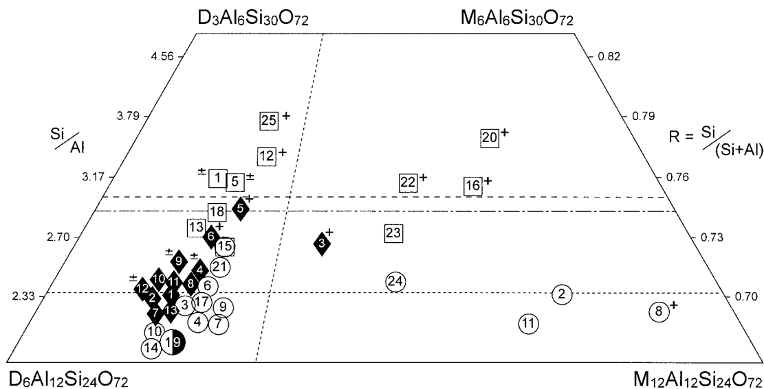
FIGURE 4. Compositional diagram showing the mean chemical analyses of the studied erionite (open circles = erionites associated with levyne; open squares = isolated erionites) and offretite (solid diamonds) samples. The sample numbers correspond to those listed in Table 1. Discrimination lines as in Figure 1. Optical sign of elongation is adjacent to each symbol: No mark means negative elongation sign, (+) means positive elongation sign, (±) means sample with crystals having positive or negative elongation sign (see text for details).
