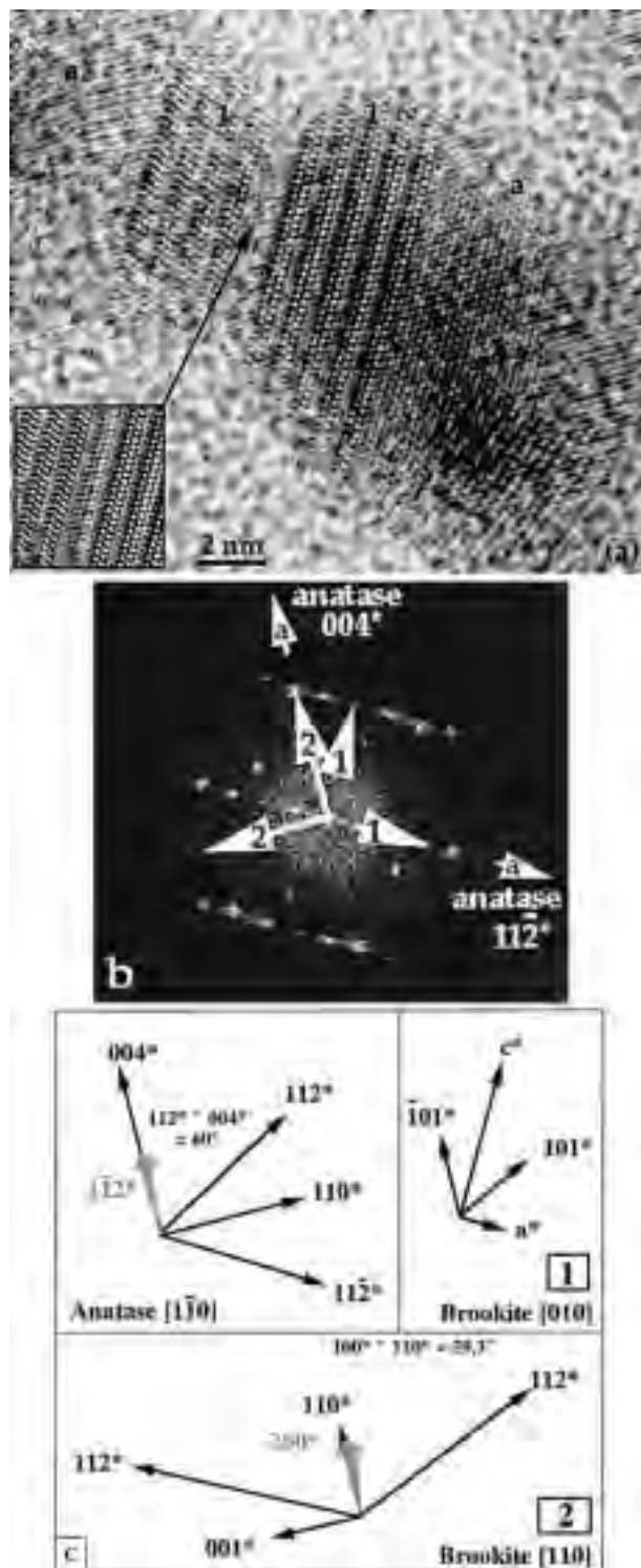
FIGURE 4. (a) HRTEM images of particles viewed down [110] anatase. Brookite in orientation “1” is viewed down [010] and “2” down [110]. Inset shows the rotationally filtered contact region (probably brookite). (b) FFT of the area in (a). (c) diagrams of the reciprocal lattices (from anatase “a” and brookite “1” and “2”). Note that brookite “2” also has (200) parallel to anatase {112}.
