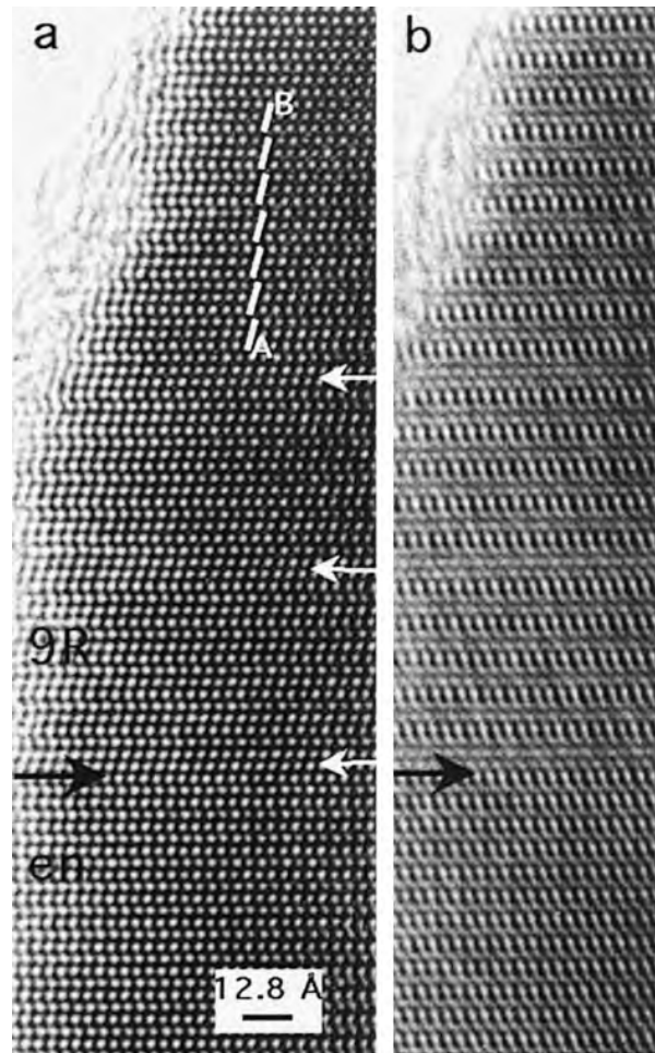
FIGURE 9. Intergrowth between enargite and a 9R polytype. The (a) and (b) images were taken at different defocus values. The black arrows mark the boundary between enargite and 9R, the white arrows indicate faults in the 9R sequence.
