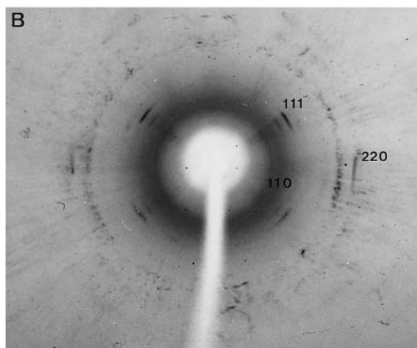
FIGURE 4. Two [110] precession photographs for a single crystal of synthetic low- and high-form pentlandites with \text{Fe}_{4.56}\text{Ni}_{4.44}\text{S}_{7.95} at 25 and 620 °C, respectively. A = 25 °C; B = 620 °C.
