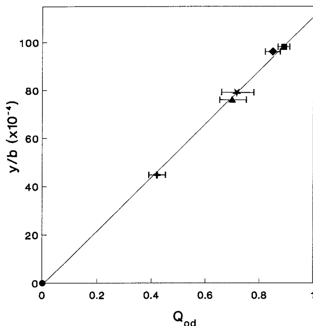
FIGURE 2. Absolute value of y/b fractional coordinate of the Pb site vs. Q_{od} . Circle and square = PbF H and PbF L , respectively (Benna et al. 1996); diamond = PbF L 1h; star = PbF L 16h; triangle = PbF L 64h; cross = PbF H 136h.
