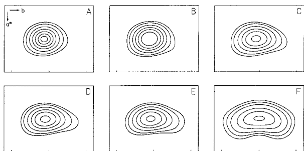
FIGURE 1. Electron-density maps for the Pb site viewed along the c axis; scale = 1 Å. (A) PbF L (Benna et al. 1996). (B) PbF L 1h. (C) PbF L 16h. (D) PbF L 64h. (E) PbF H 136h. The contours drawn correspond to 20, 40, 80, 130, 180, and 240 e - Å -3 . (F) PbF H (Benna et al. 1996). The coordinates of the center of the plots are: x = 0.27 , y = 0 , z = 0.07 for A, B, C, D, E, and z = 0.14 for F.
