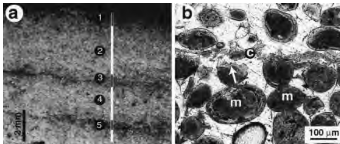
FIGURE 3. (a) Binocular photomicrograph showing the microbial mat analyzed for the present study. Five distinct layers are visible: Layer 1, which is un lithified, is caramel colored; Layers 3 and 5, which are crusty, are gray-green; and Layers 2 and 4, also un lithified, are white. Sample 6/97.NS.8n, Highborne Cay, Bahamas. (b) Thin section photomicrograph showing the
