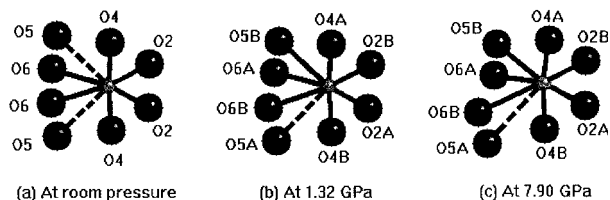
FIGURE 5. Atomic coordination for the M4 cation in cummingtonite: (a) at room pressure, (b) at 1.32 GPa, and (c) at 7.90 GPa. The distances connected by solid lines are within 3.0 \text{ \AA} and the dashed lines beyond 3.0 \text{ \AA} .
